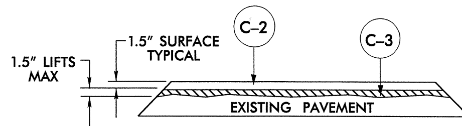
DETAIL NO. 6 LEVELING COURSE AS DIRECTED BY ENGINEER (SEE 'CONSTRUCTION NOTES')
