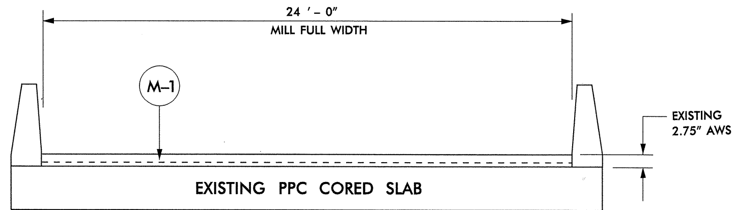
DETAIL NO. 8 Bridge No. 117, Map No. 6 Only See "2006 Bridge Data Listing" Below For Further Information
