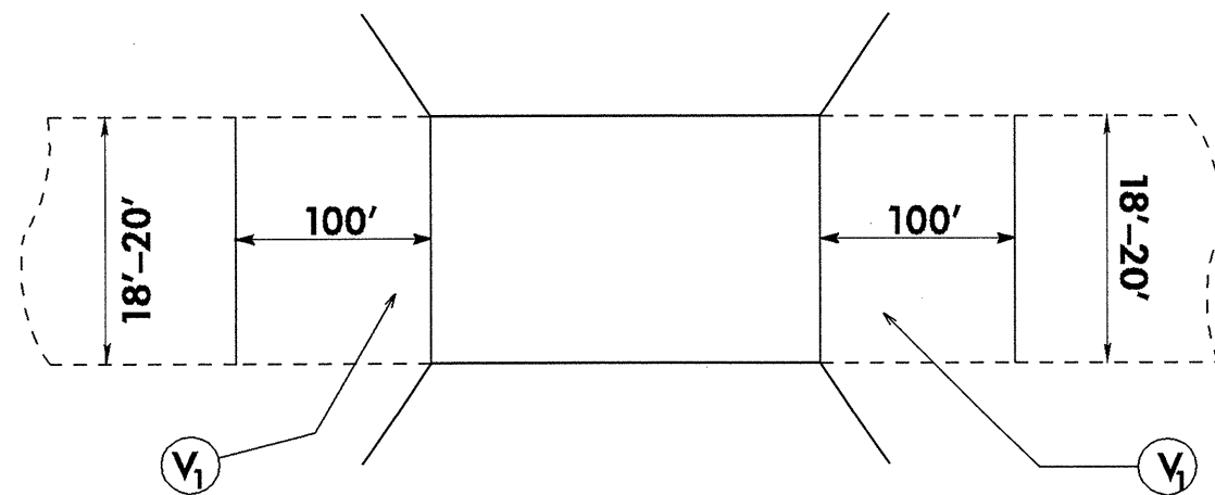
BRIDGE TYPICAL SECTION
