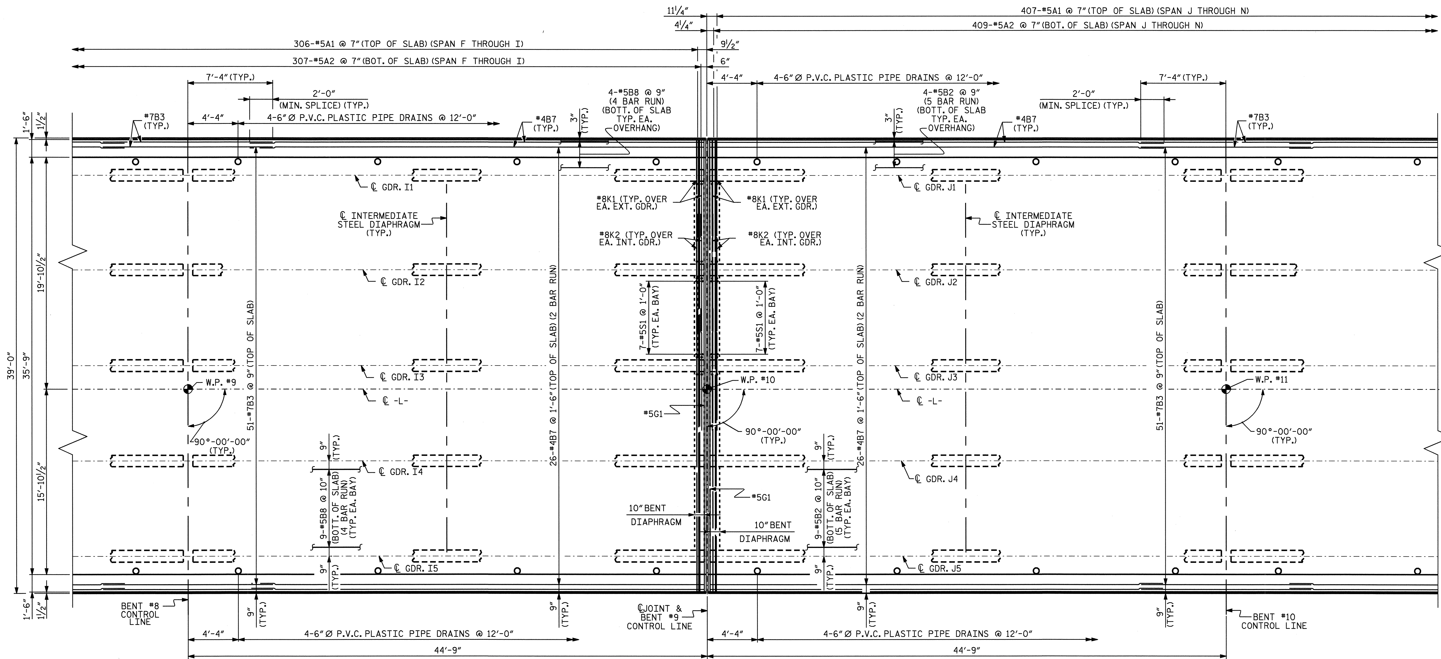
PLAN OF SPAN I
