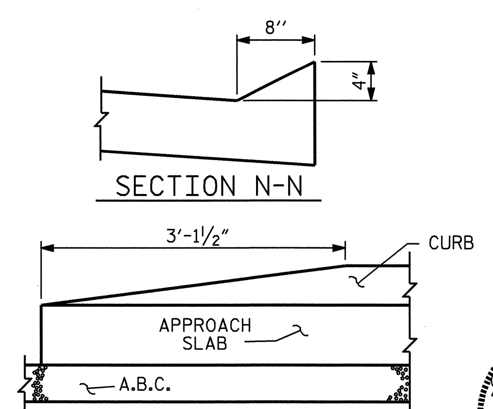
END OF CURB WITHOUT SHOULDER BERM GUTTER
