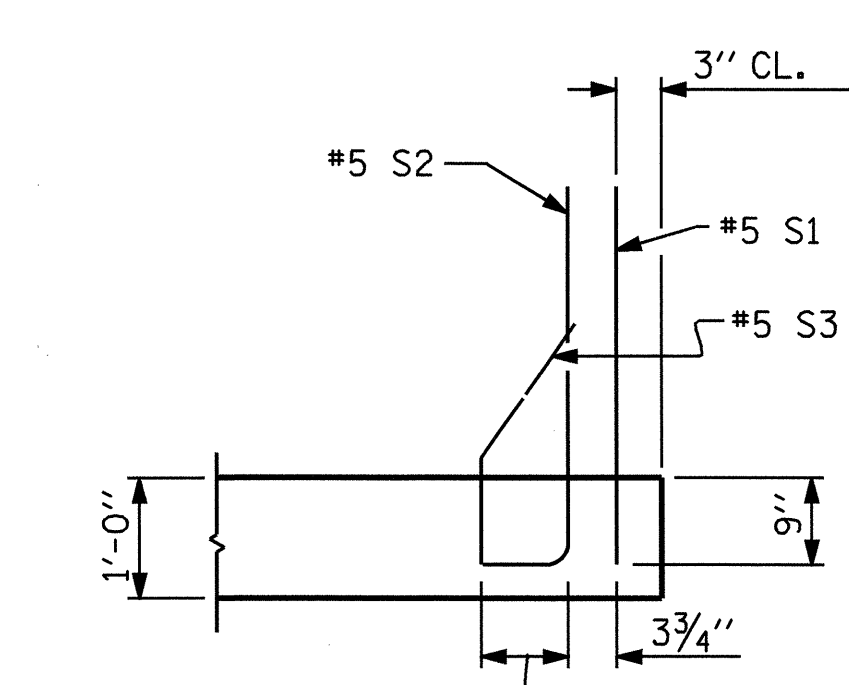
SECTION L-L
