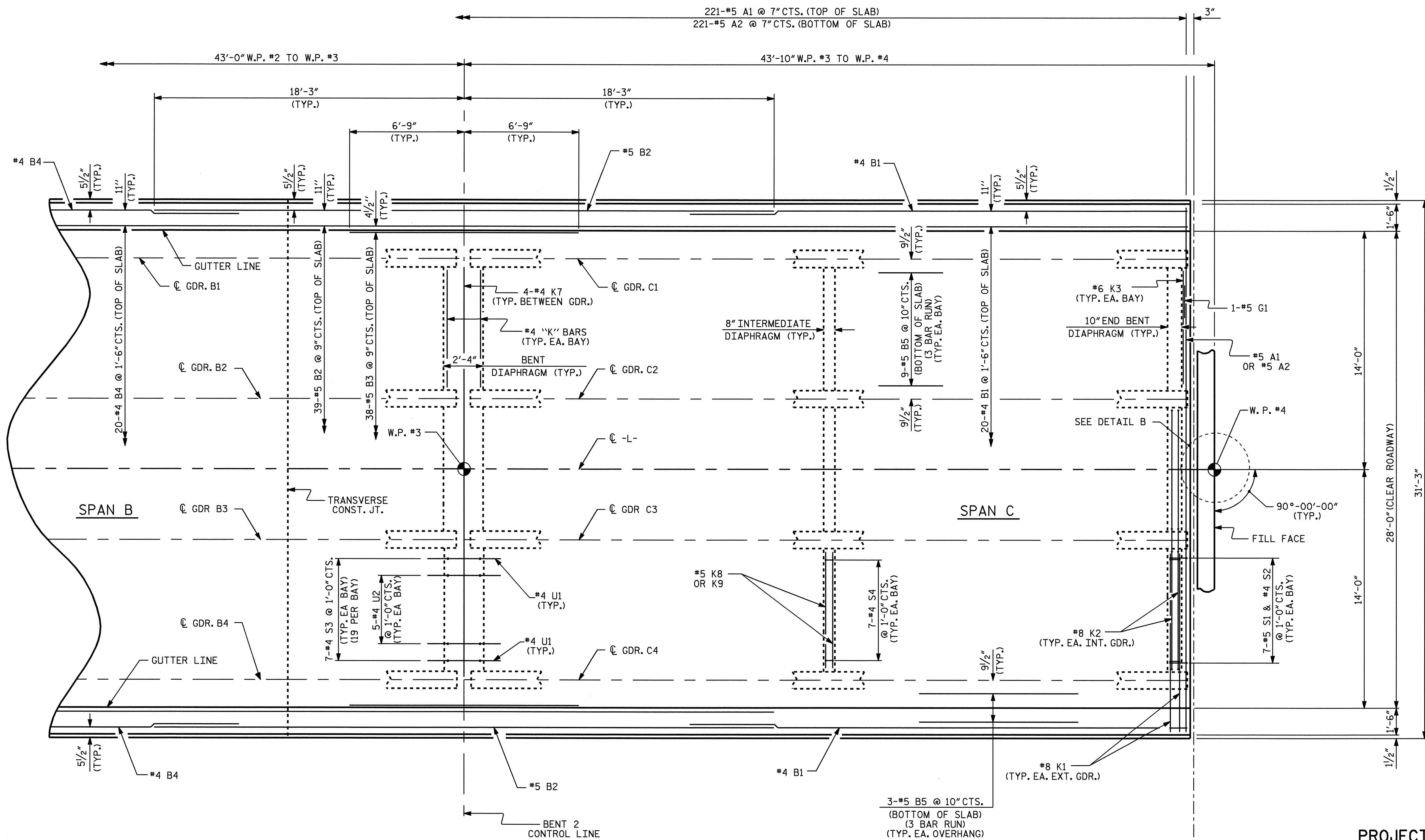
PLAN OF SPANS
