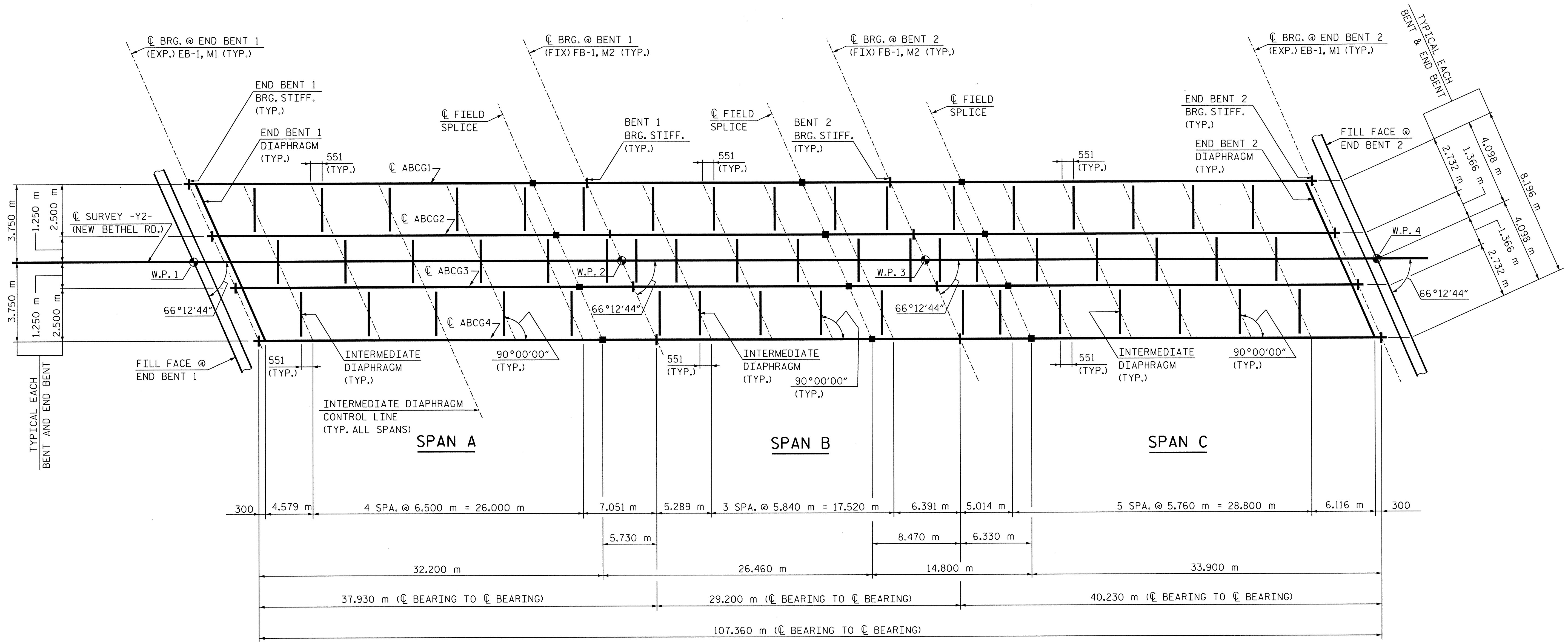
CONTINUOUS GIRDER FRAMING PLAN NOTE: GIRDERS ARE STRAIGHT AND PARALLEL TO ONE ANOTHER.
