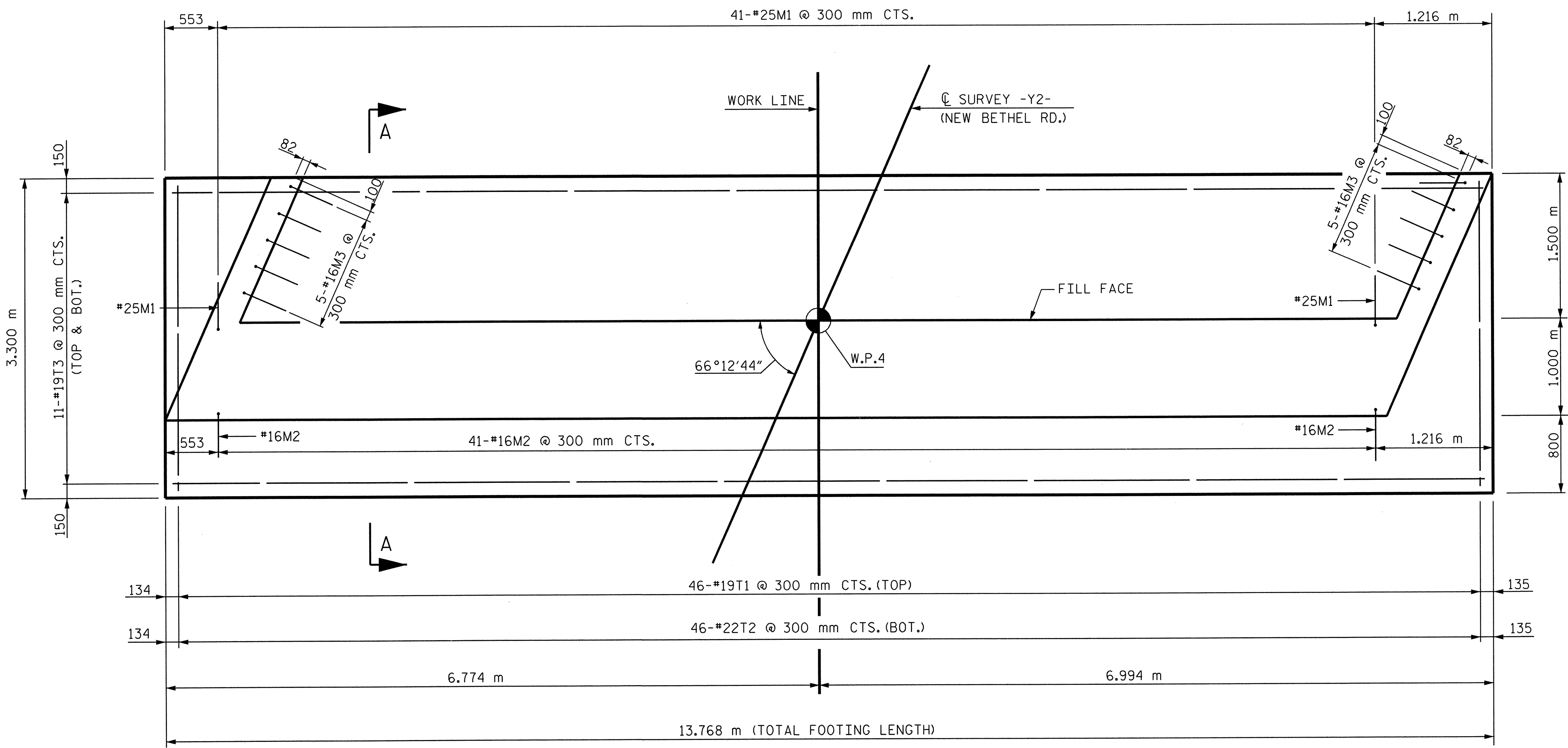
PLAN
