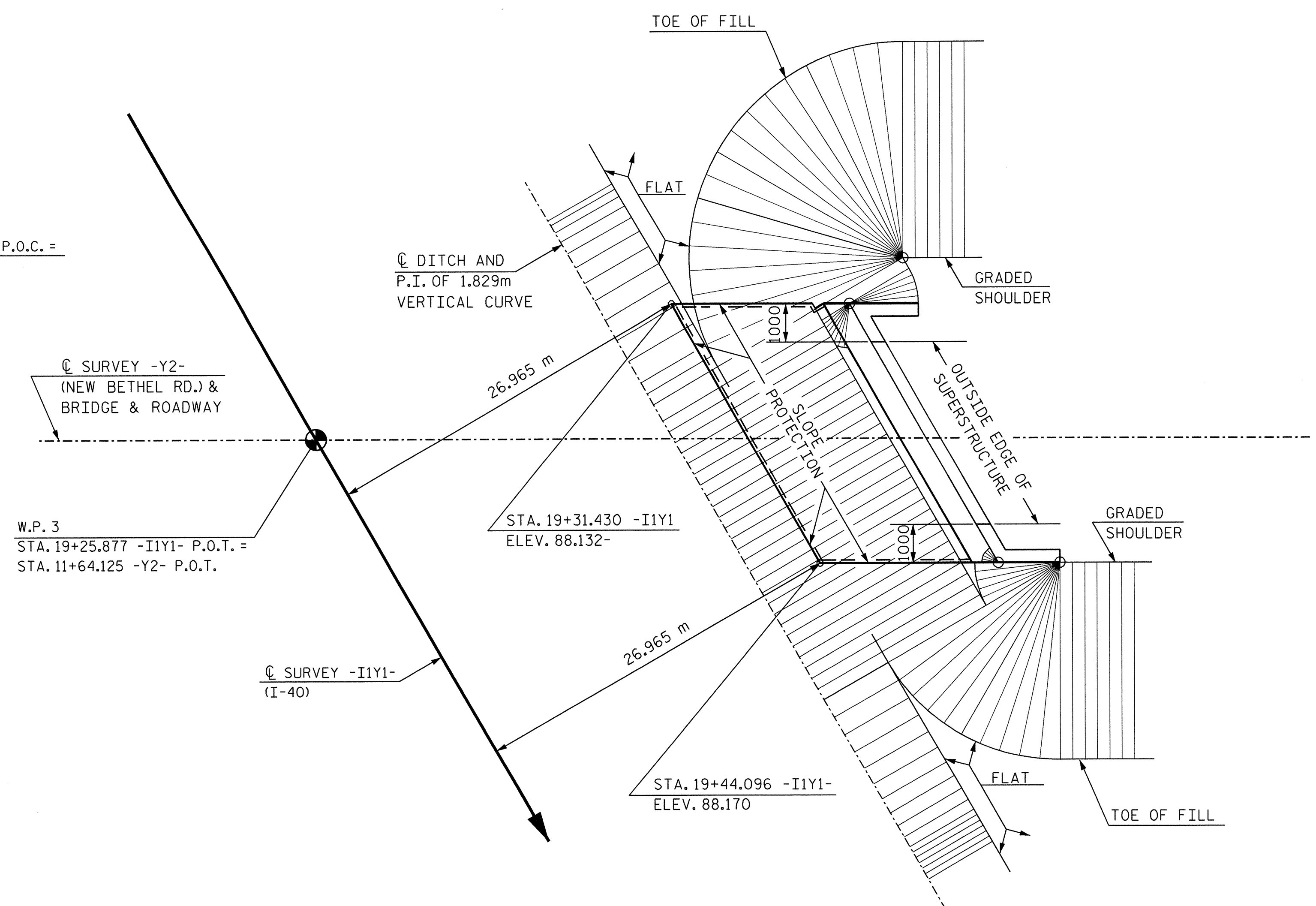
PLAN - END BENT 2 WITH SWEEP BACK WINGS - SKEWED (2:1 SLOPE)
