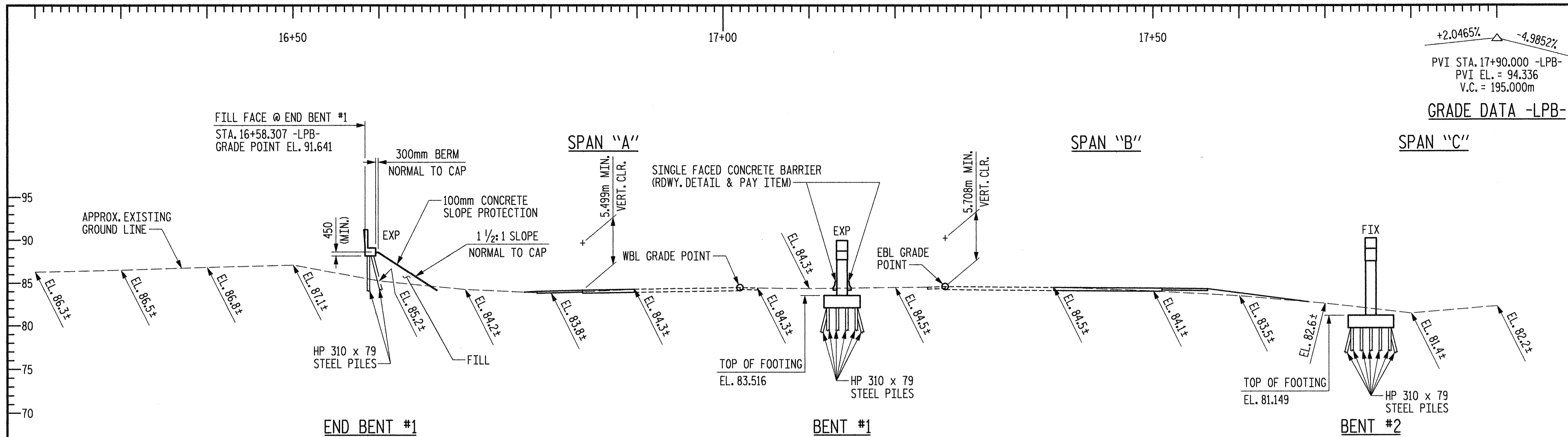
SECTION ALONG Q SURVEY -LPB- (BENTS ON SECTION AT RIGHT ANGLES TO BENTS)
