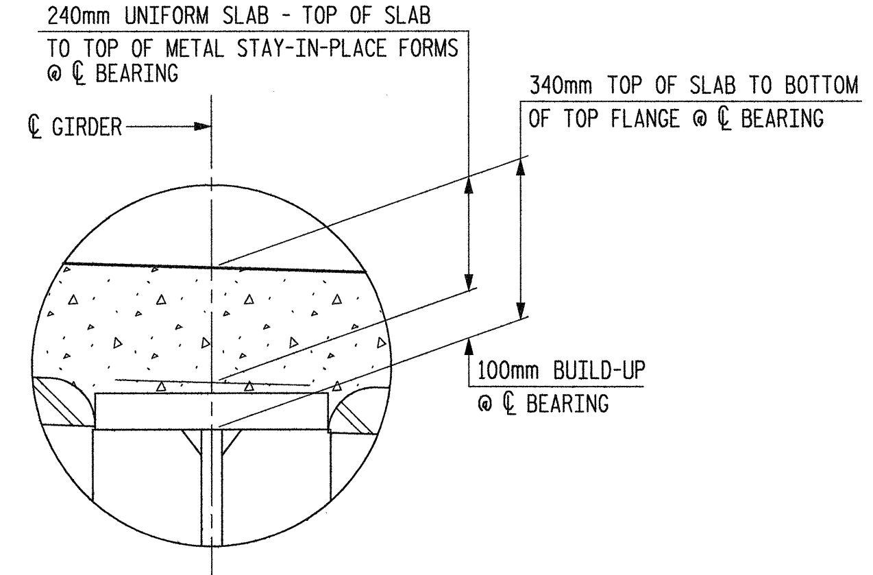
DETAIL "A"
