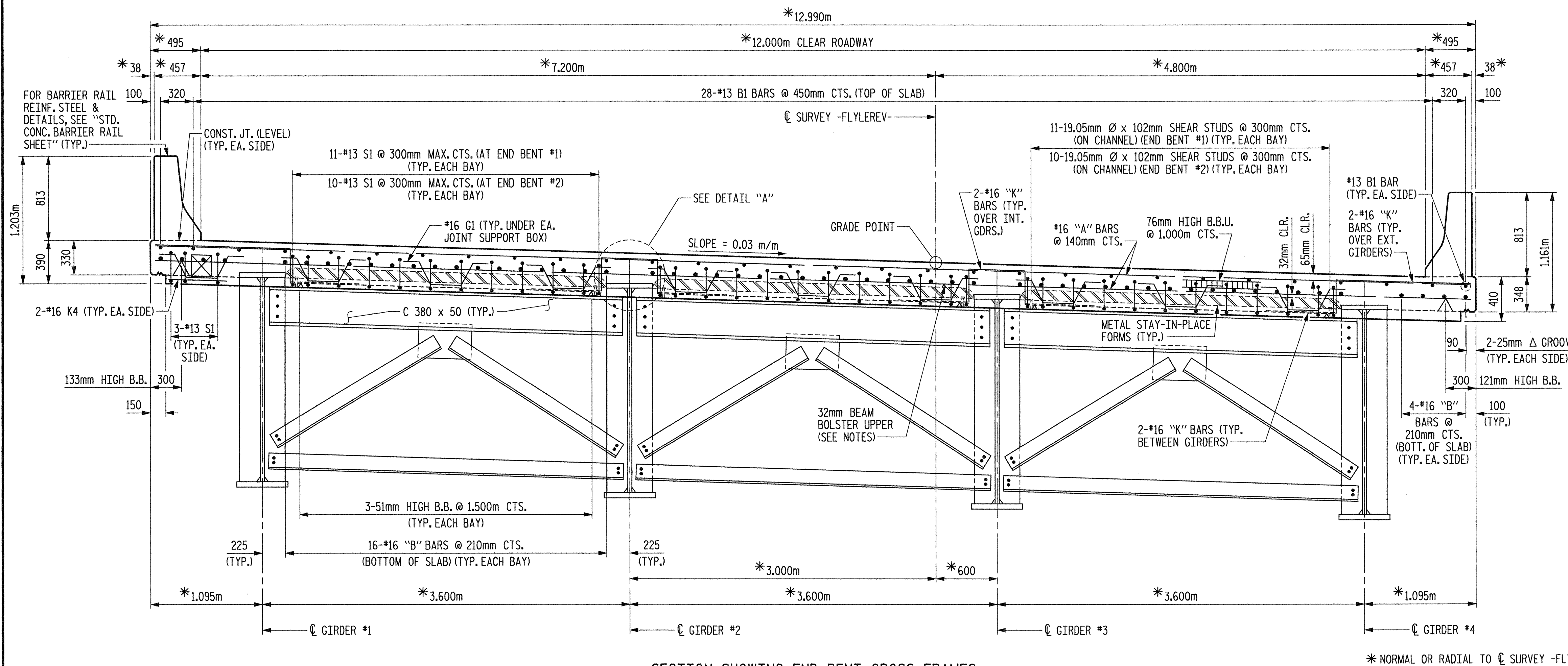
SECTION SHOWING END BENT CROSS FRAMES FOR DETAILS, SEE "DROPWALL DETAILS AT END BENT CROSSFRAME" ON SHEET 2 OF 2.
