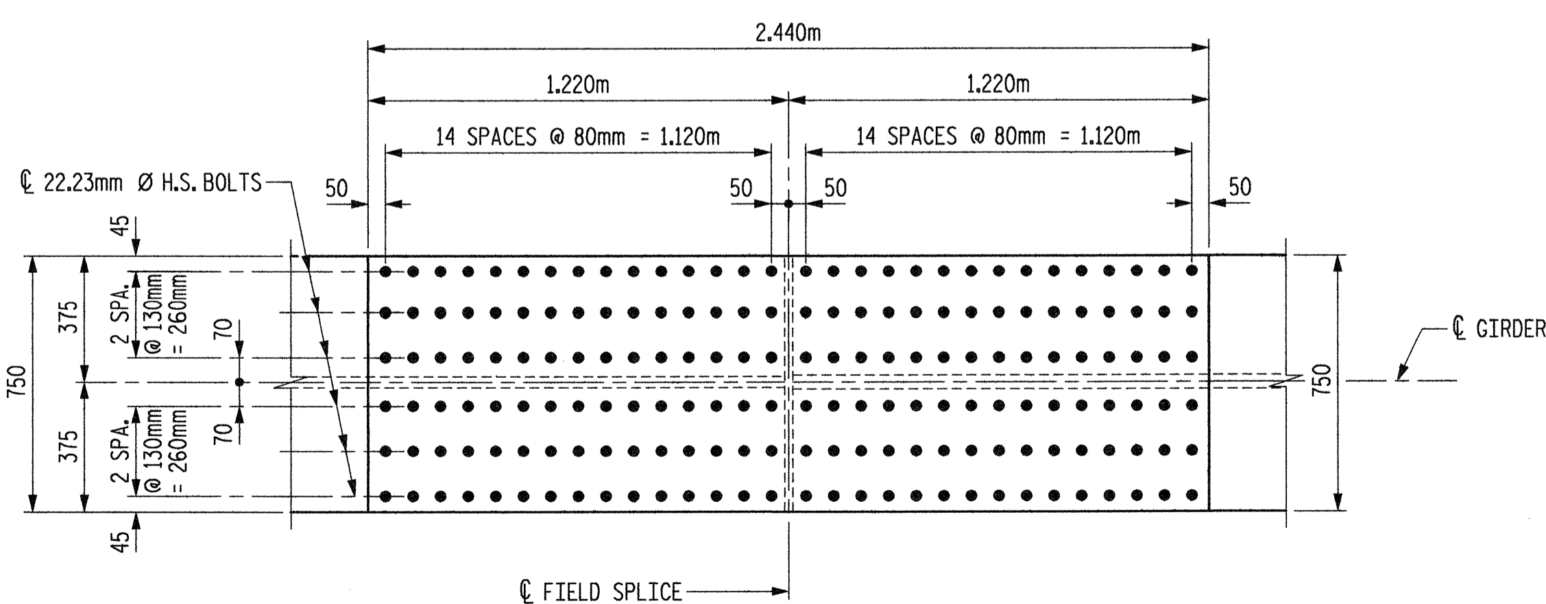
FIELD SPLICE DETAILS - FS4
