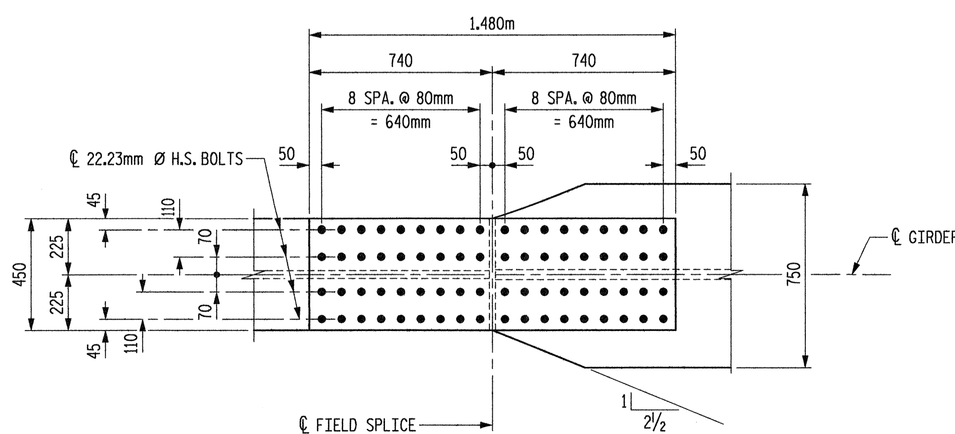
FIELD SPLICE DETAILS - FS3
