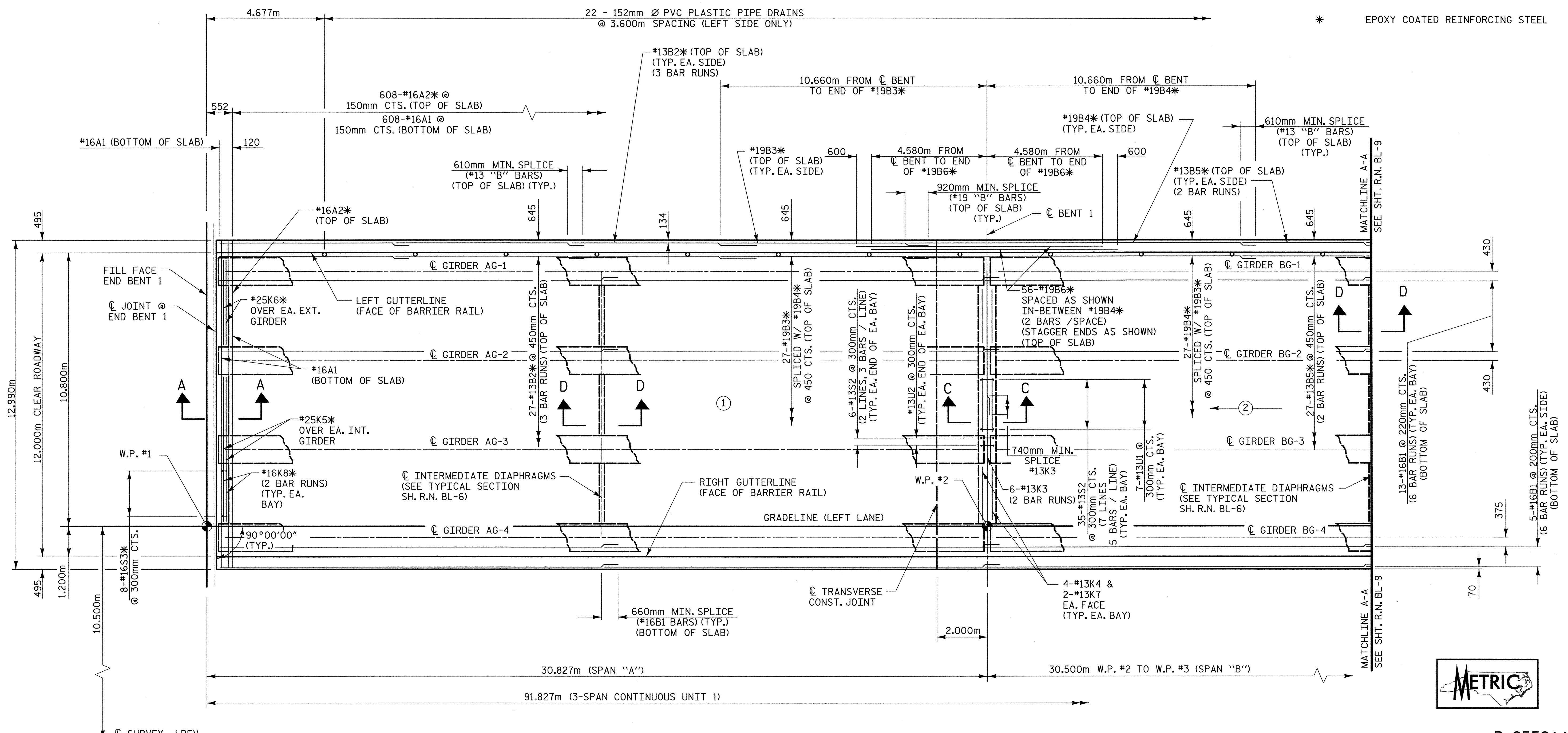
PLAN - UNIT 1
