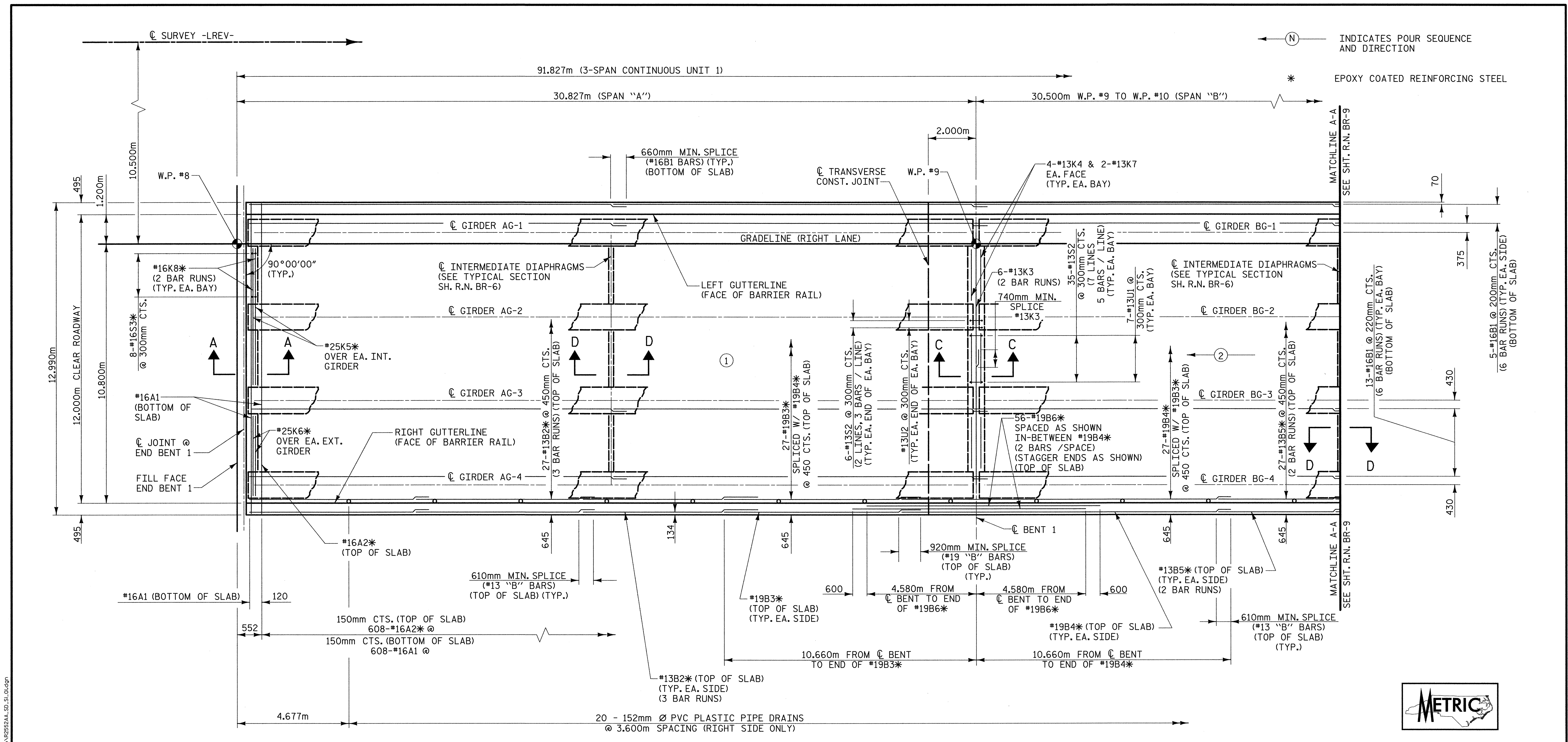
PLAN - UNIT 1
