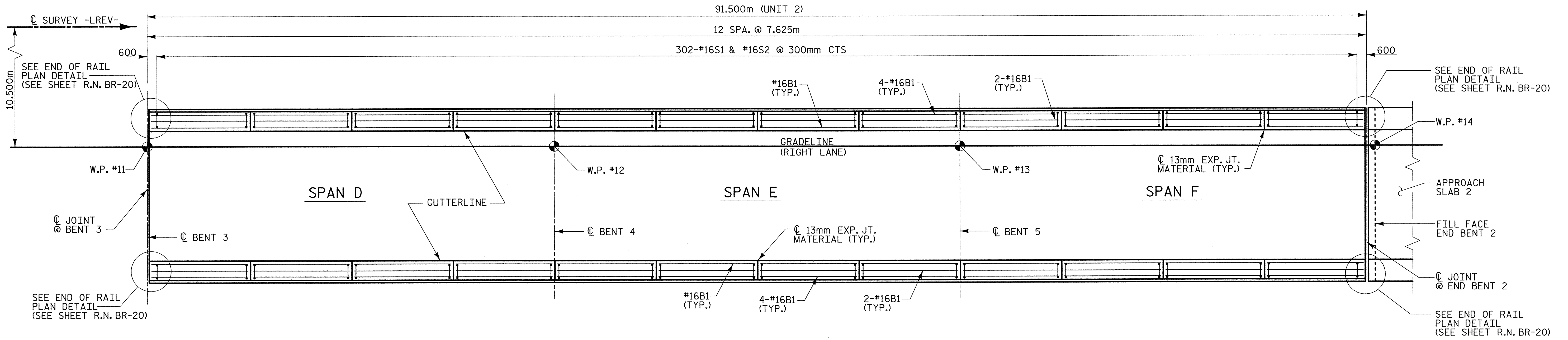
PLAN SPANS D-F
