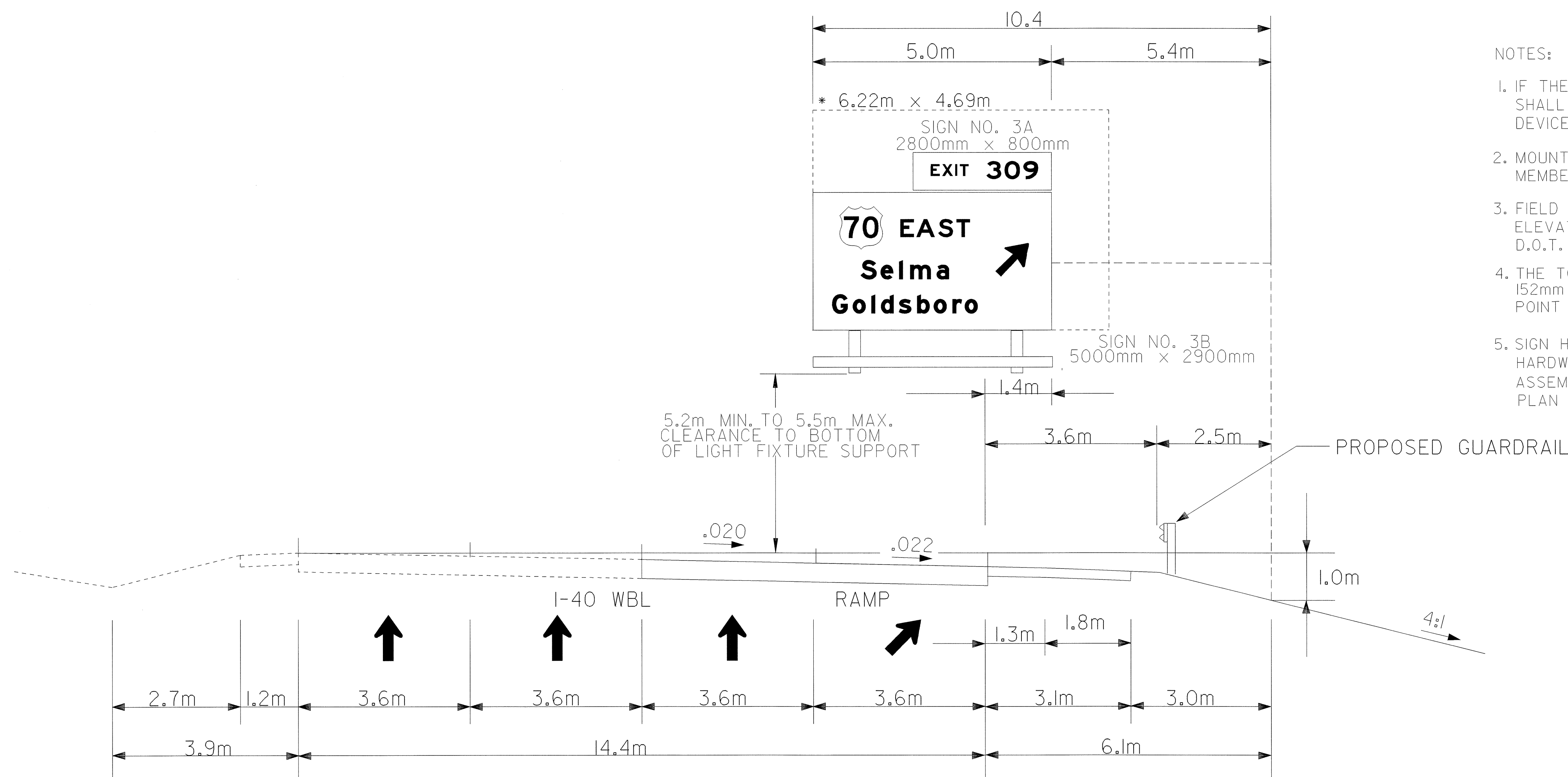
OVERHEAD SIGN ASSEMBLY "B" I-40 WESTBOUND
