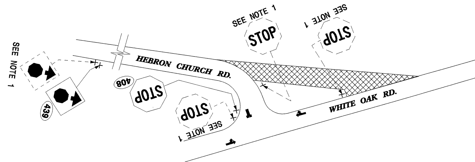
DETAIL OF IMPROVEMENTS TO THE INTERSECTION OF WHITE OAK RD. AND HEBRON CHURCH RD.
