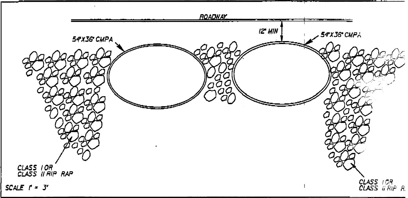
TYPICAL CROSS SECTION VIEW
