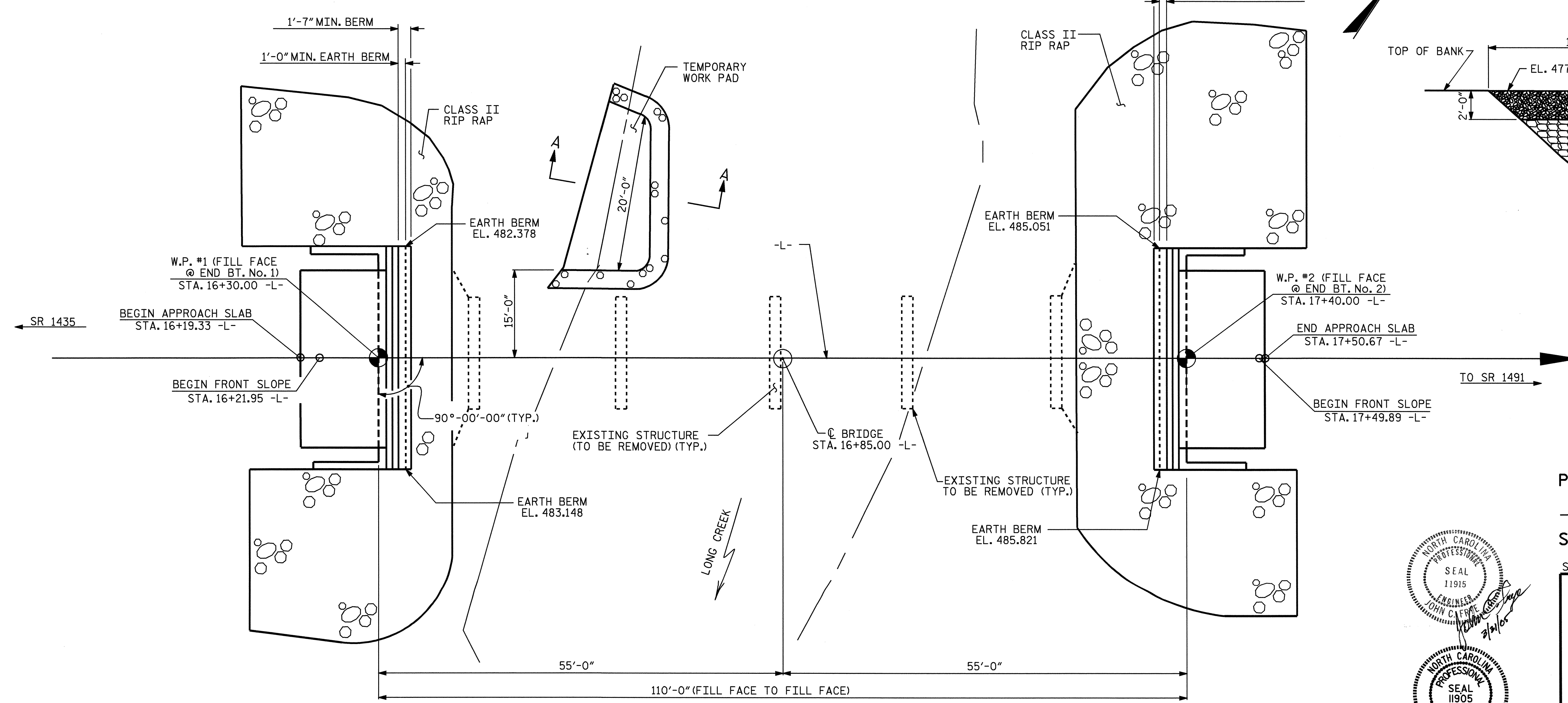
PLAN (PILES NOT SHOWN IN PLAN VIEW)
