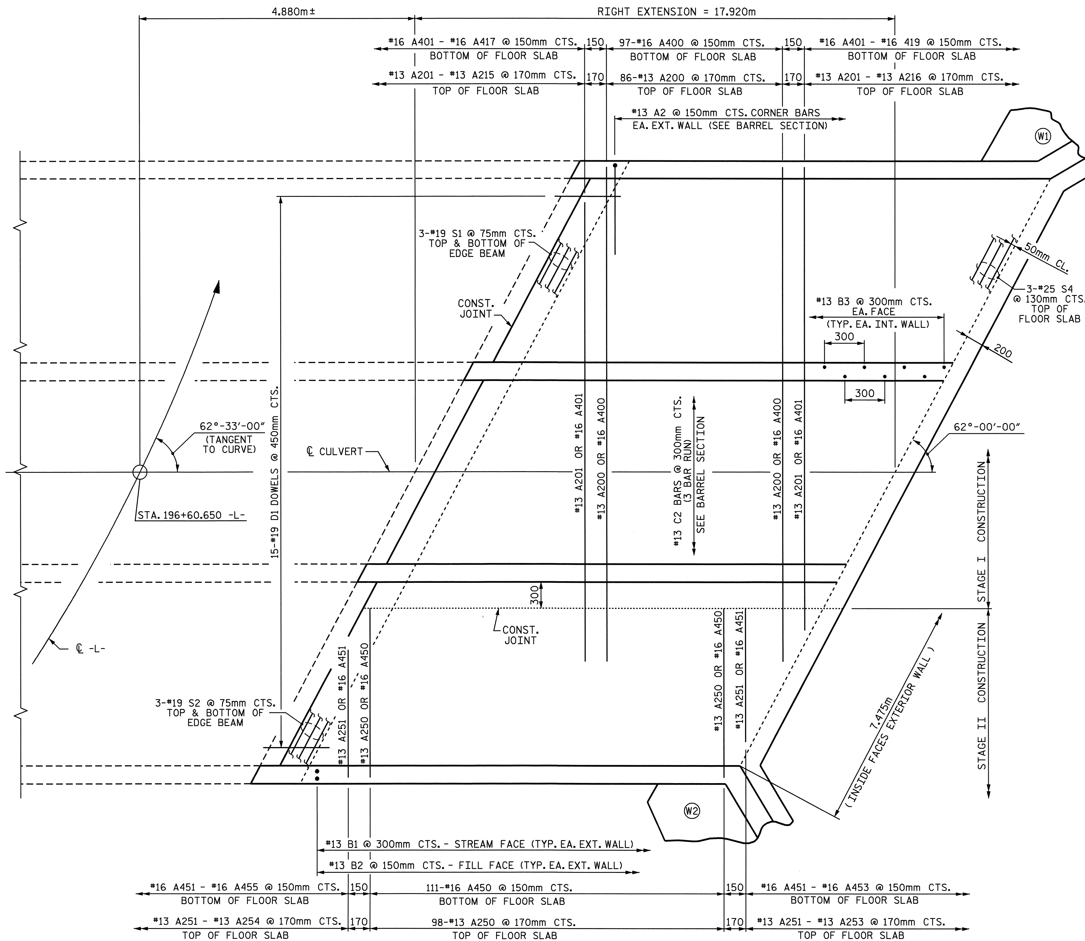
PLAN OF FLOOR SLAB
