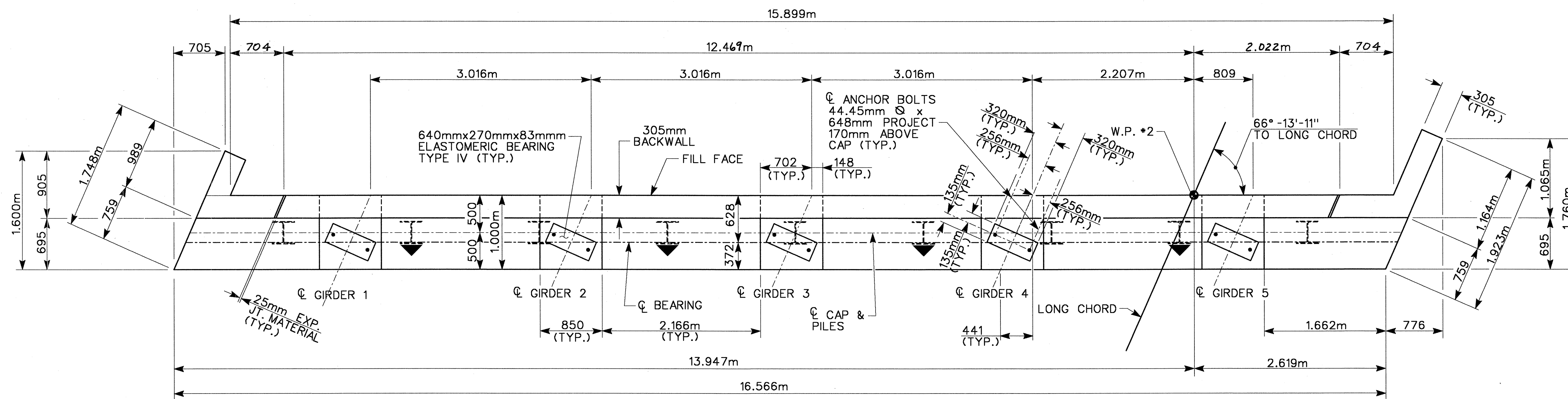
PLAN
