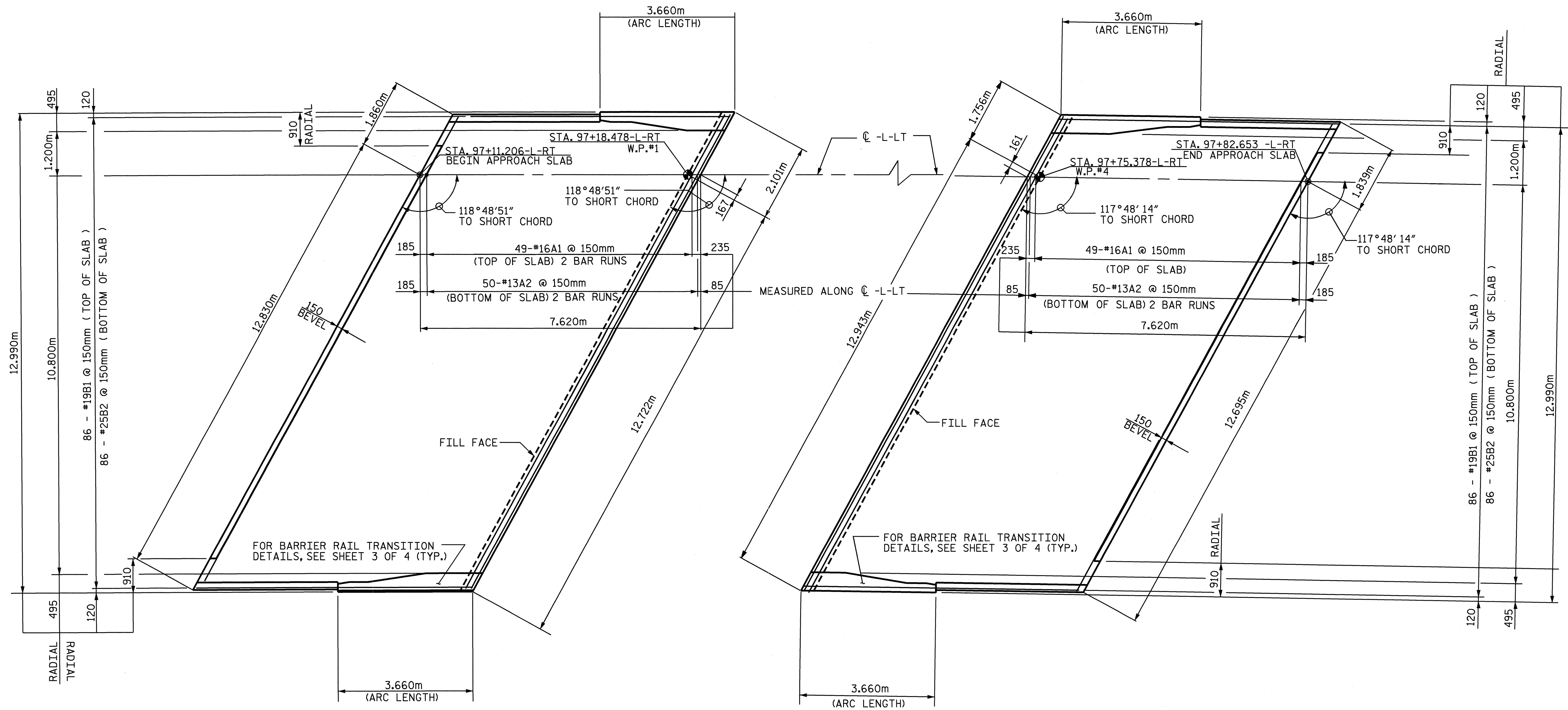
APPROACH SLAB @ END BENT 2
