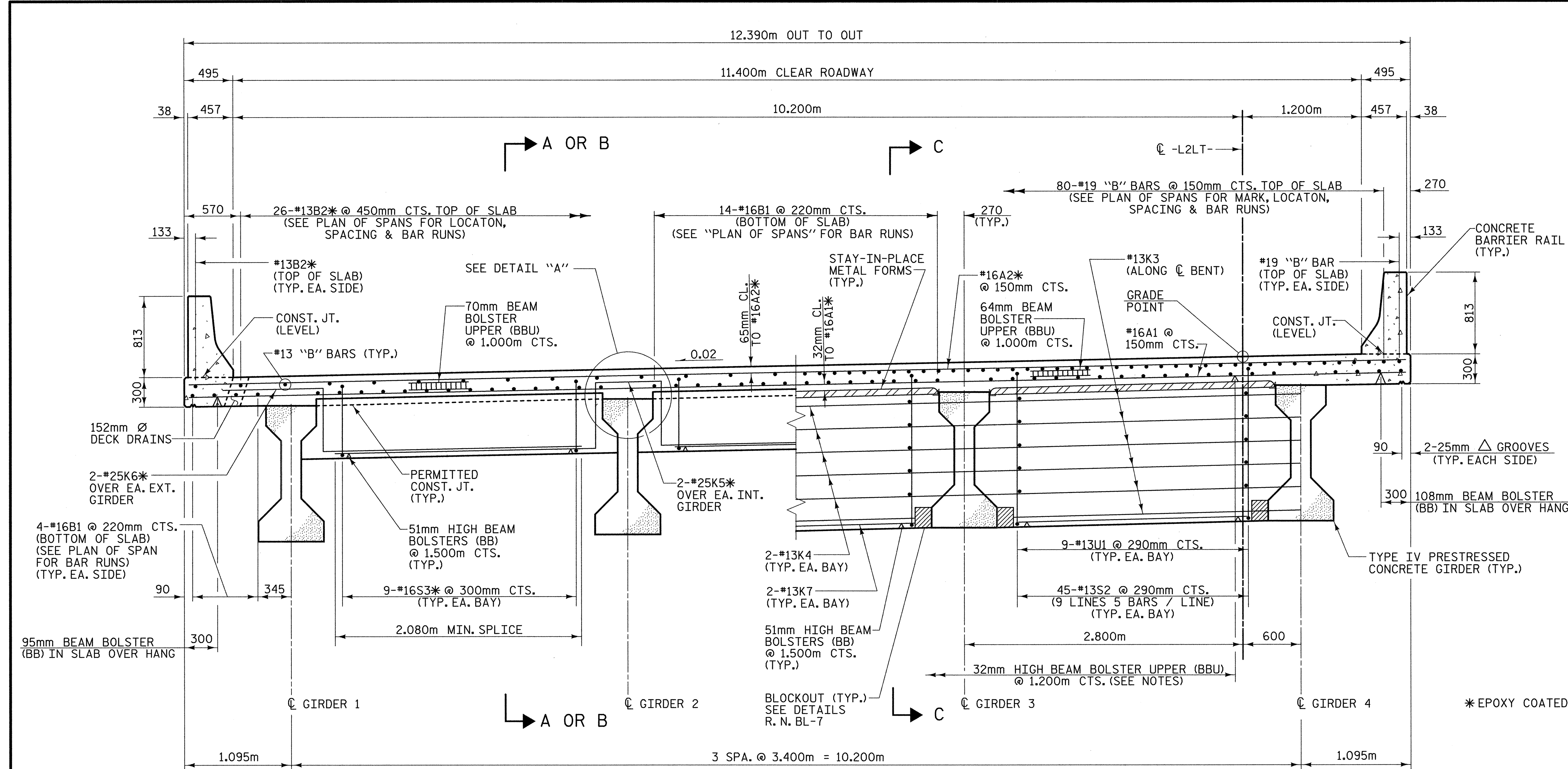
HALF SECTION AT EXPANSION DIAPHRAGMS END BENTS 1 & 2, & BENT 3
