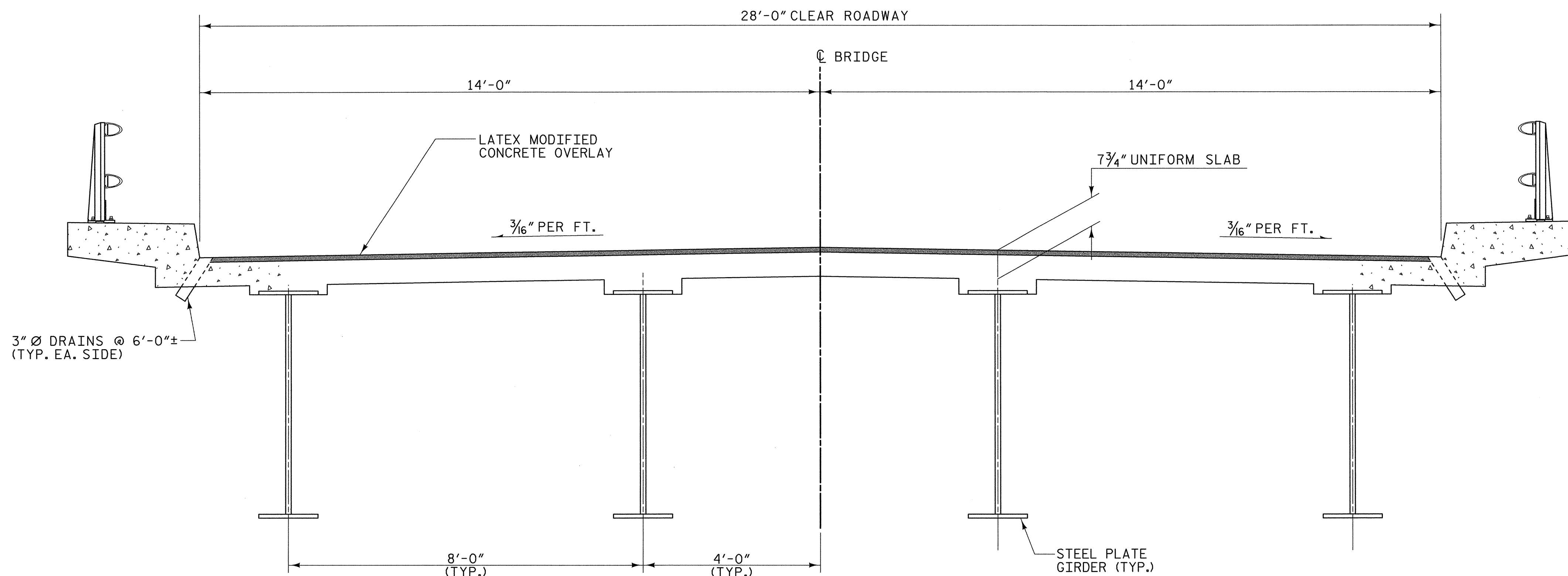
TYPICAL SECTION (SPANS 17 THRU 19)
