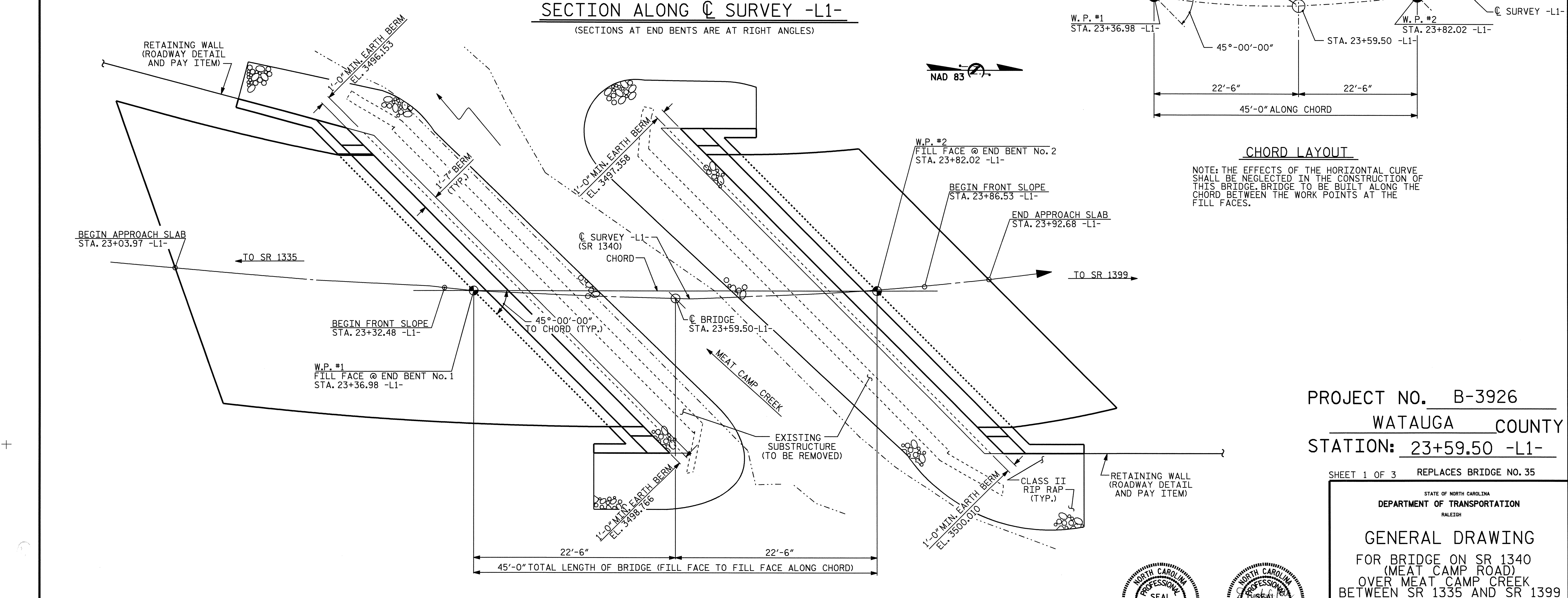
PLAN (PILES FOR END BENTS ARE NOT SHOWN FOR CLARITY)
