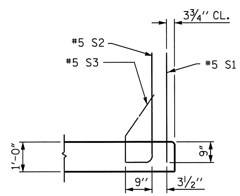
SECTION K-K
