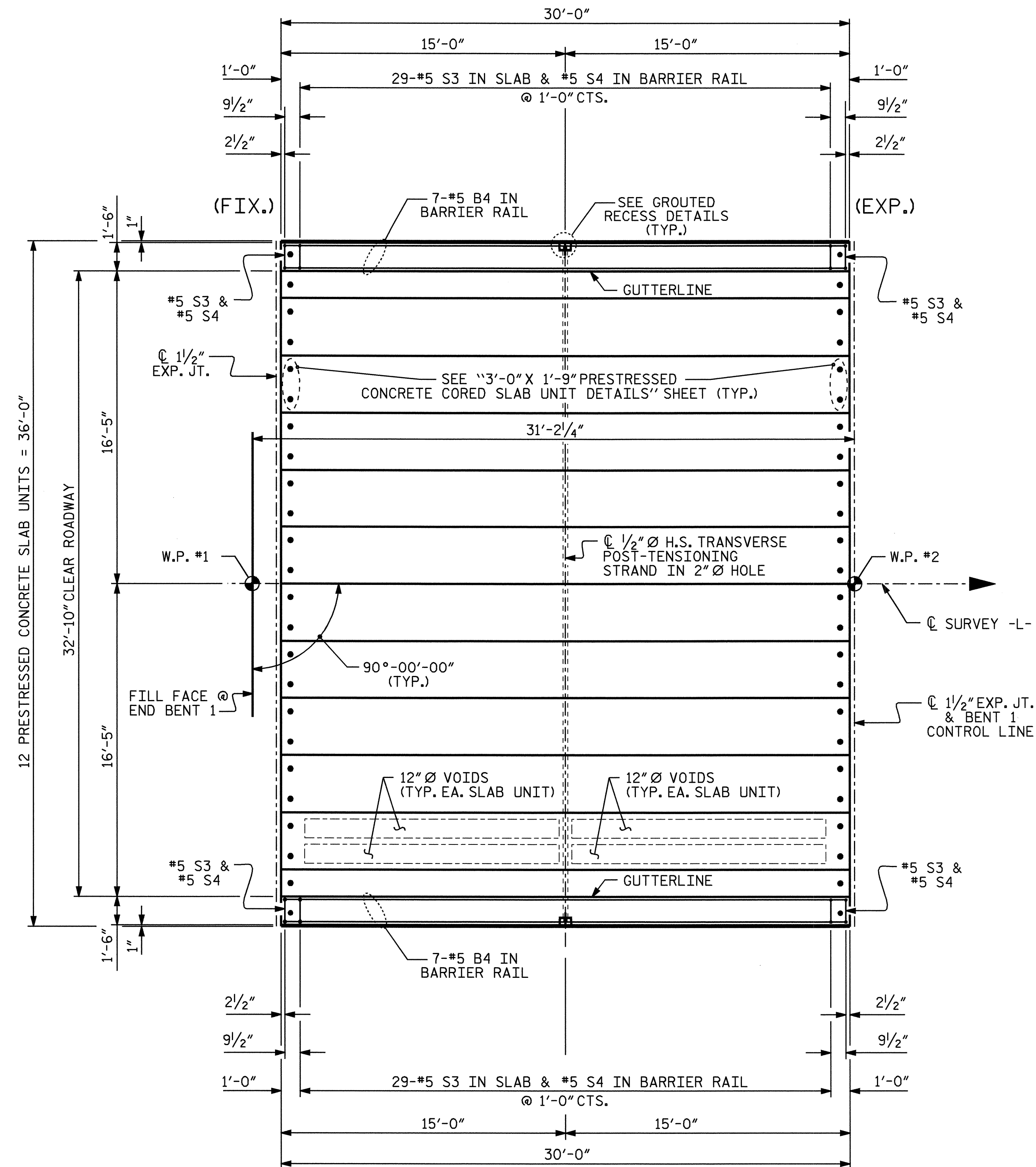
PLAN OF SPAN A
