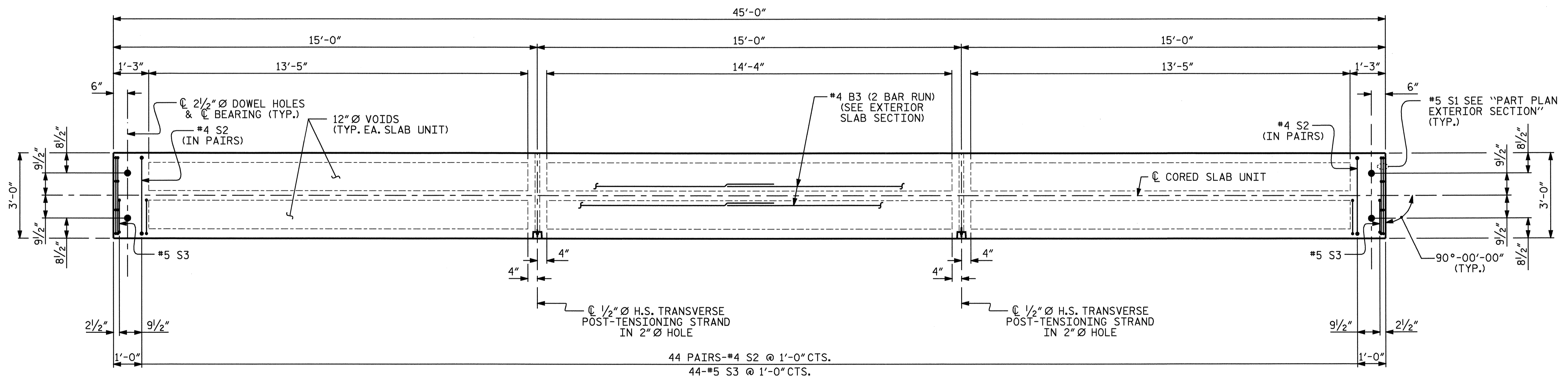
PLAN OF EXTERIOR SLAB
