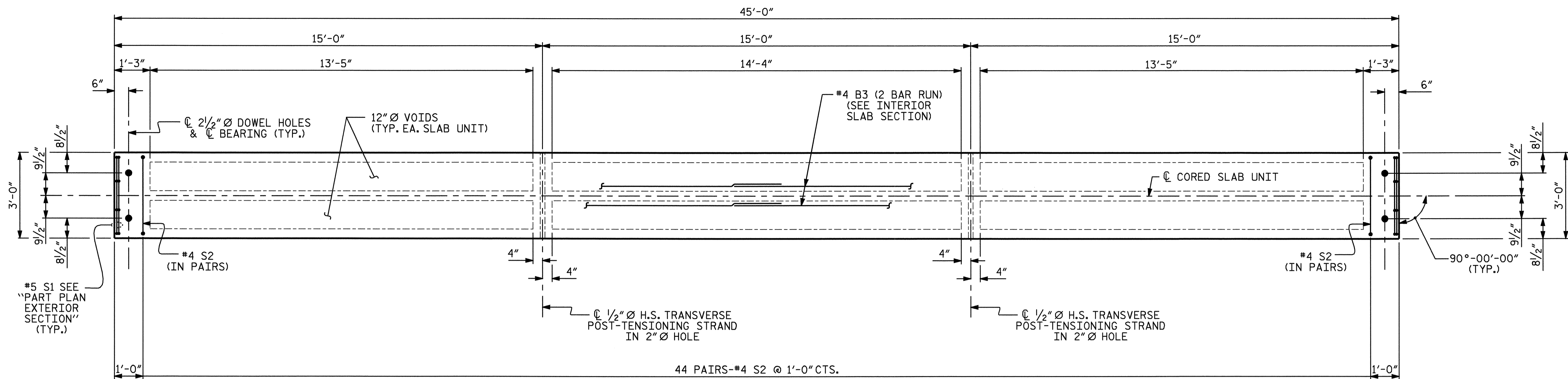
PLAN OF INTERIOR SLAB
