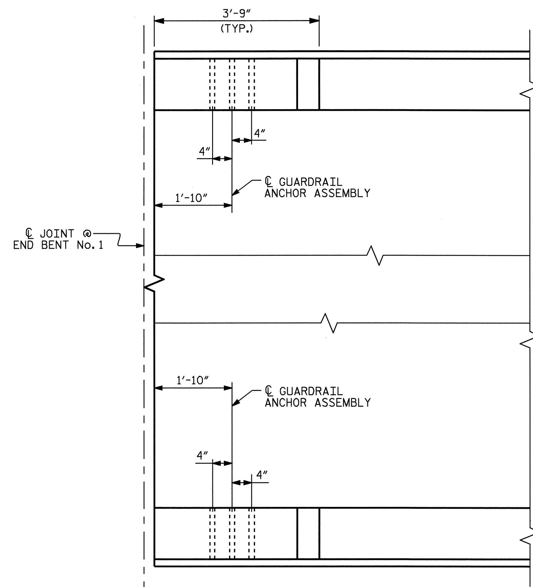
PLAN (END BENT No. 1 SHOWN, END BENT No. 2 SIMILAR)
