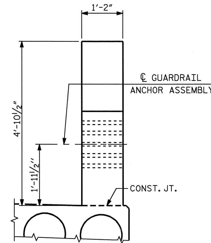
END VIEW (TWO BAR METAL RAIL)
