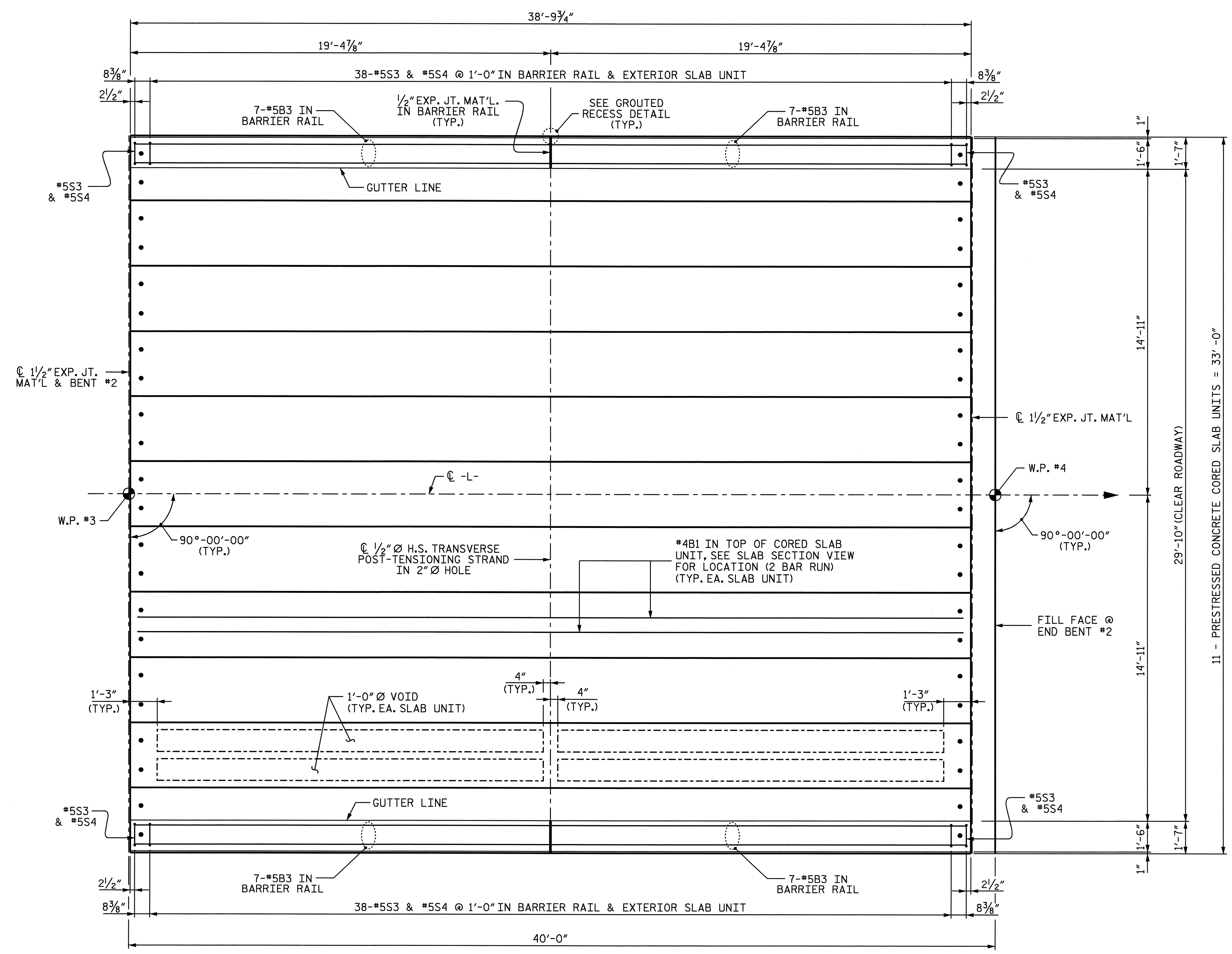
PLAN OF SPAN C
