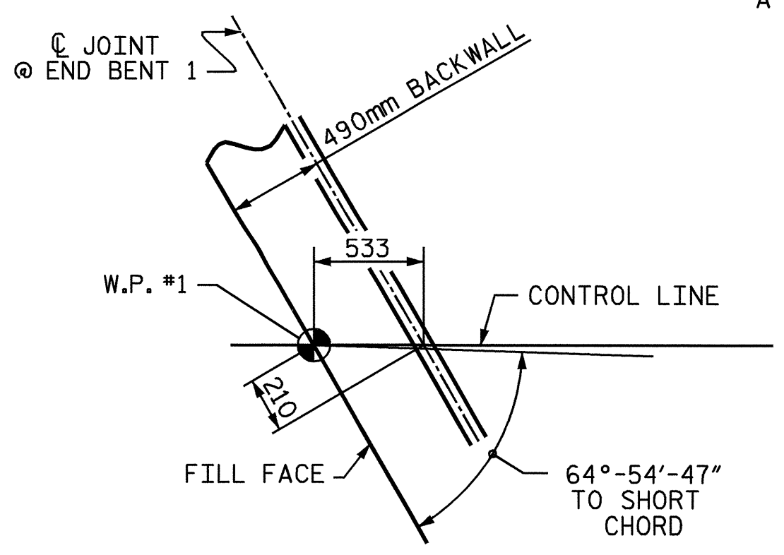
DETAIL 'A'
