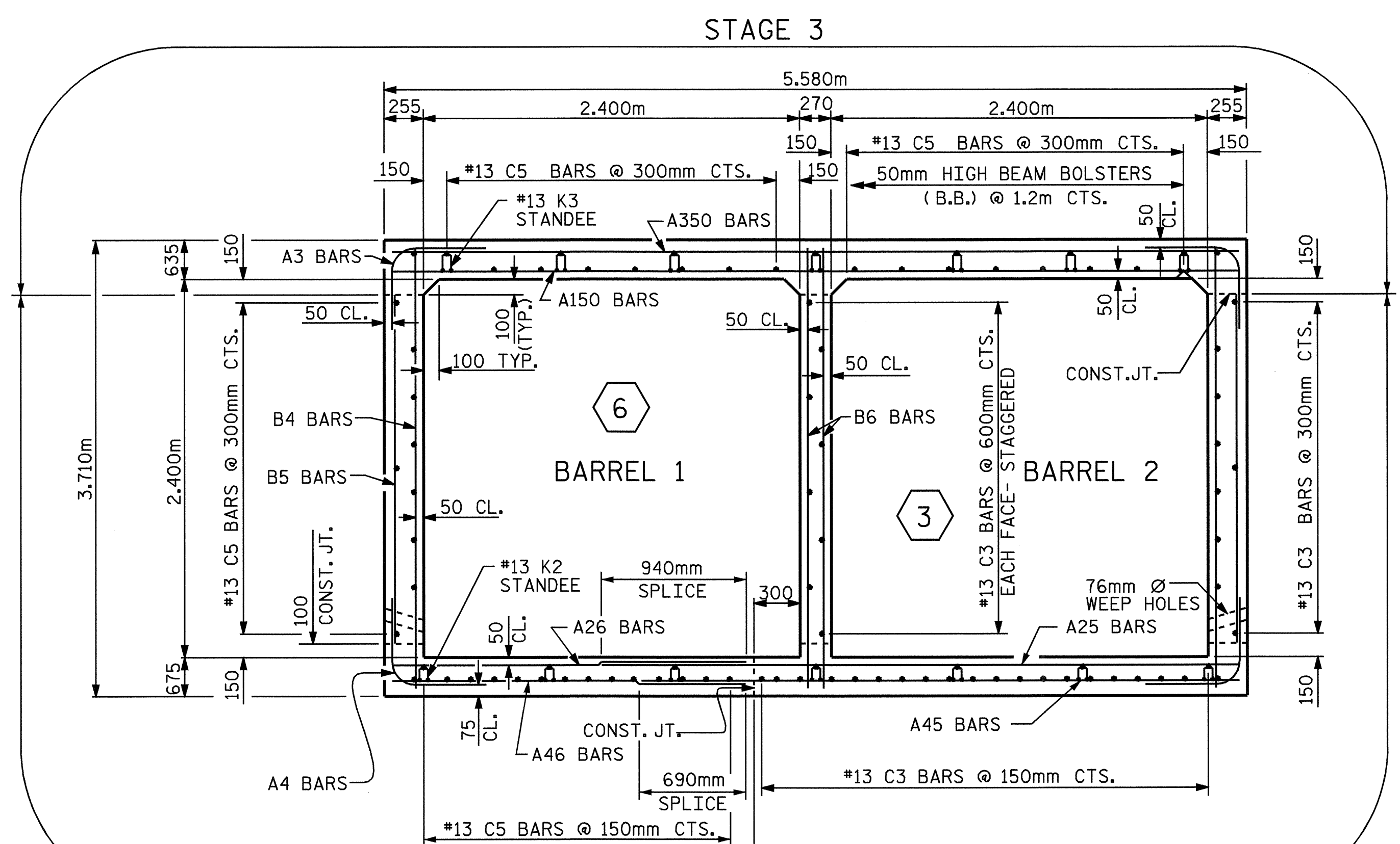
SECTION C-C (PARTS 3 & 6)
