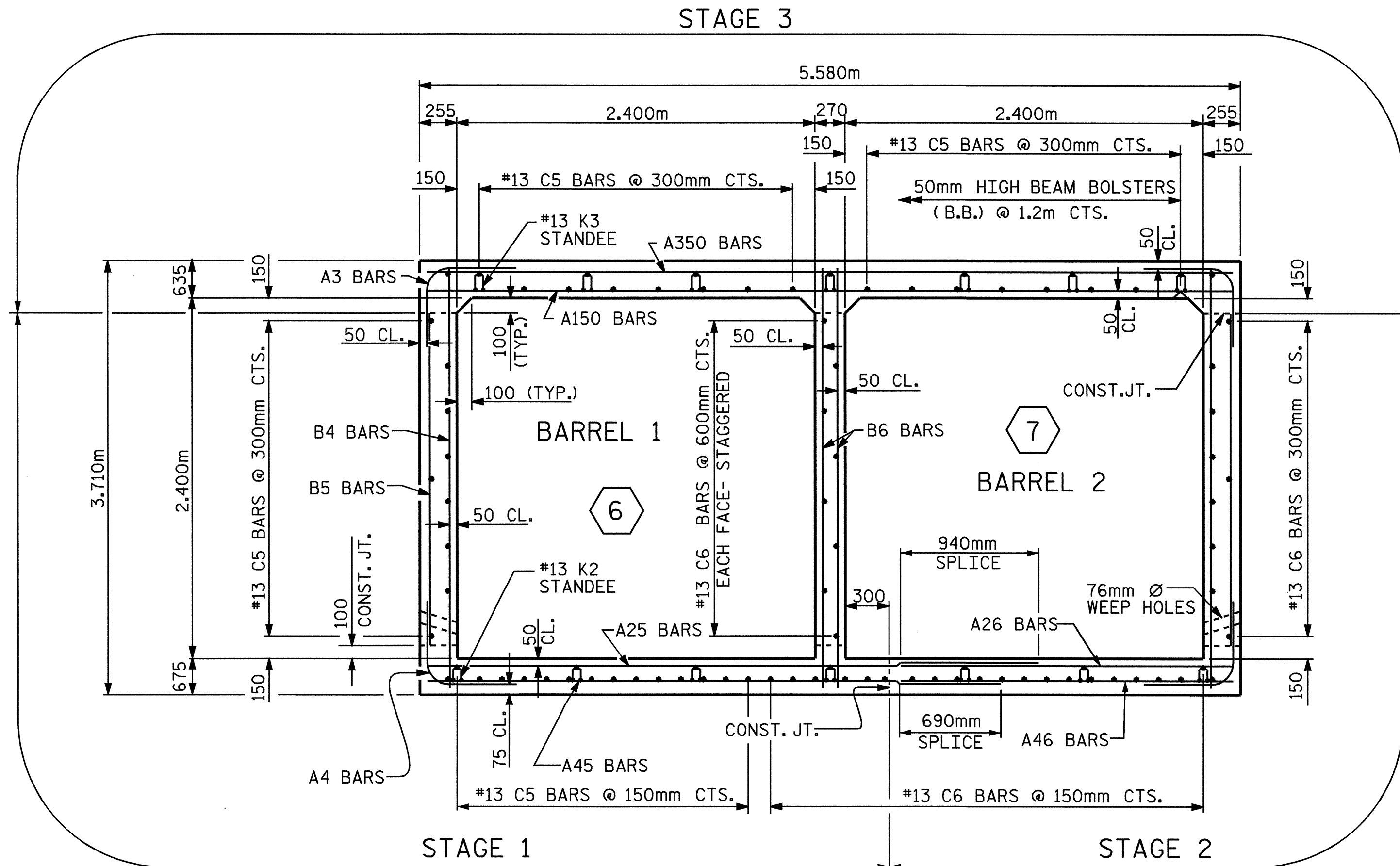
SECTION D-D (PARTS 6 & 7)
