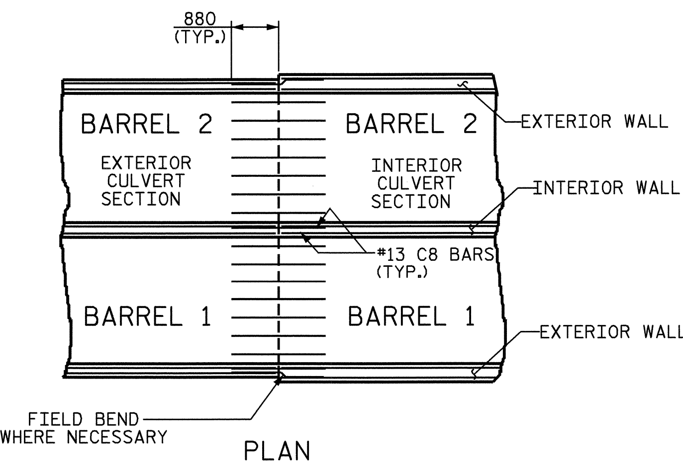
DETAIL SHOWING TYPICAL PLACEMENT OF #13 C8 BARS BETWEEN BARREL PARTS
