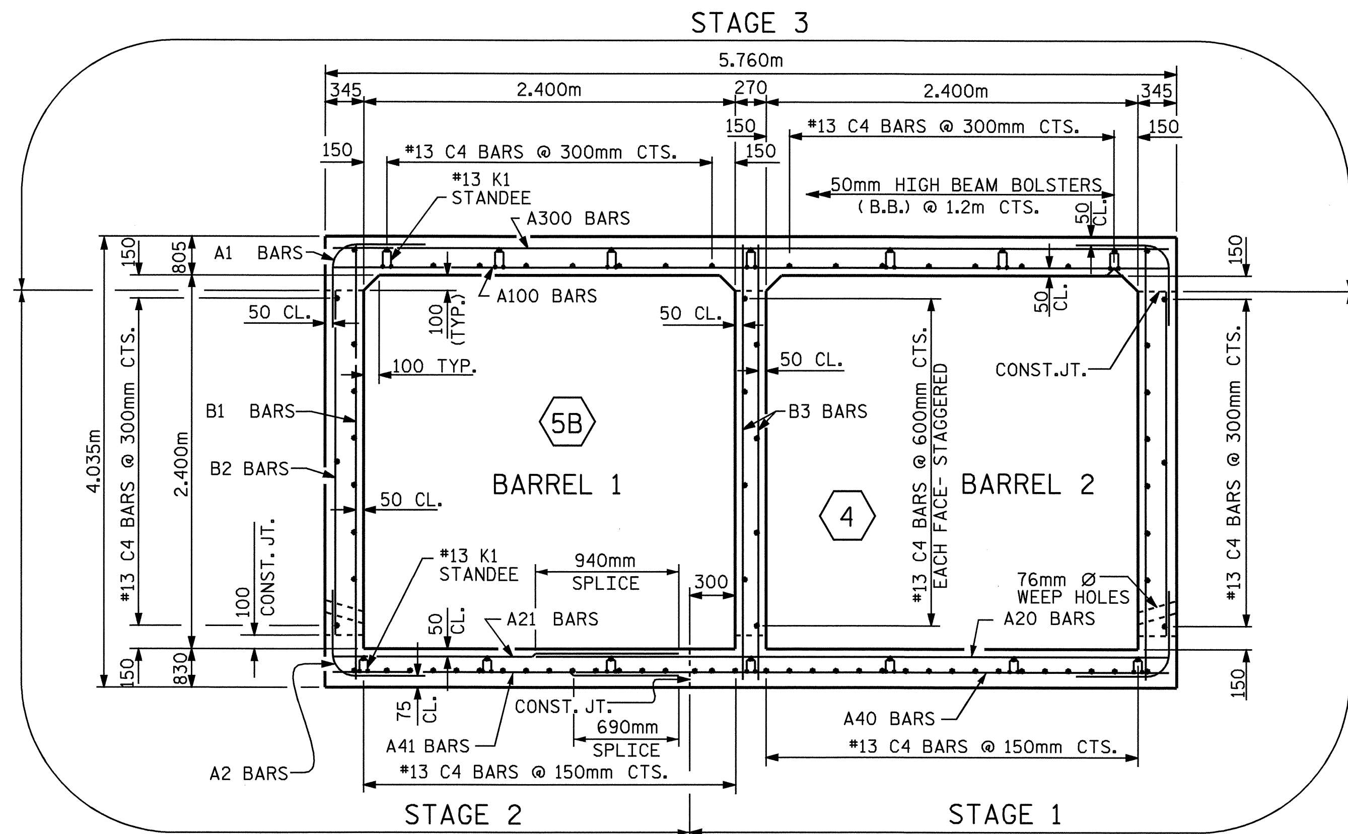
SECTION E-E (PARTS 4 & 5B)
