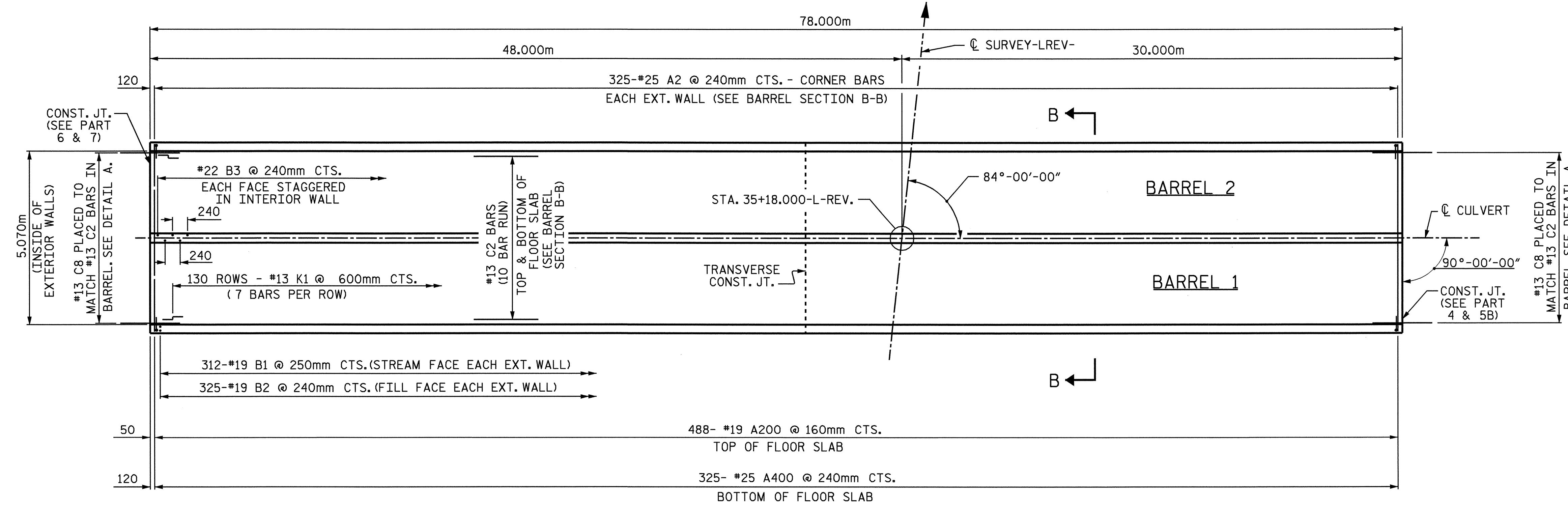
PLAN OF CULVERT - FLOOR SLAB - PART 2
