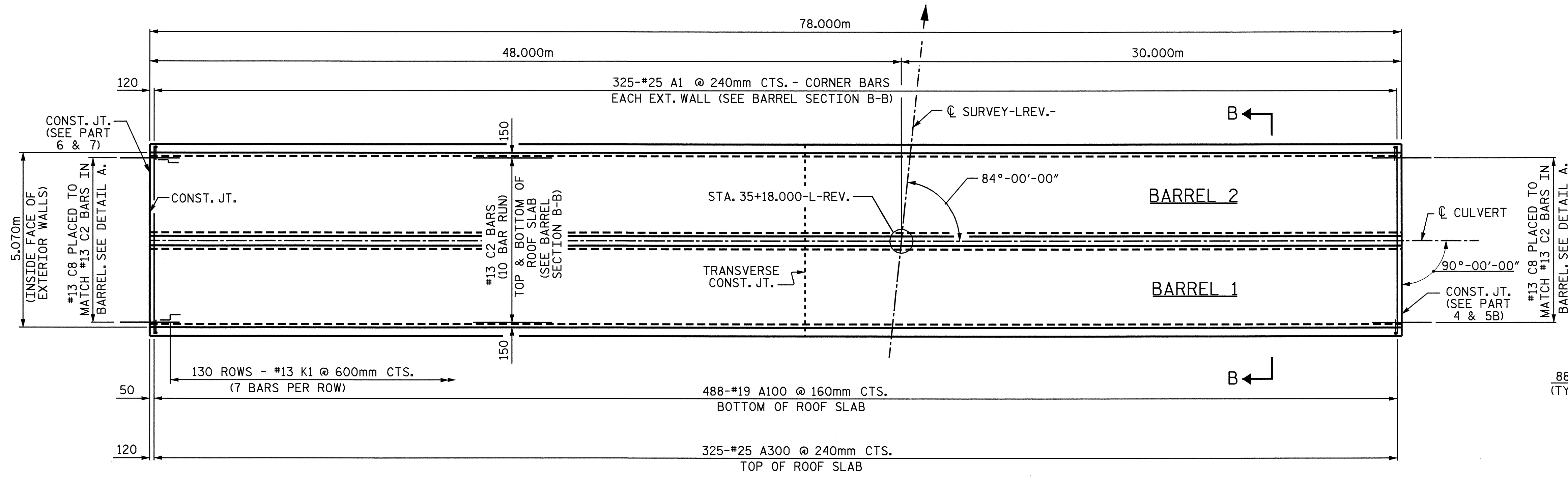
PLAN OF CULVERT - ROOF SLAB - PART 2
