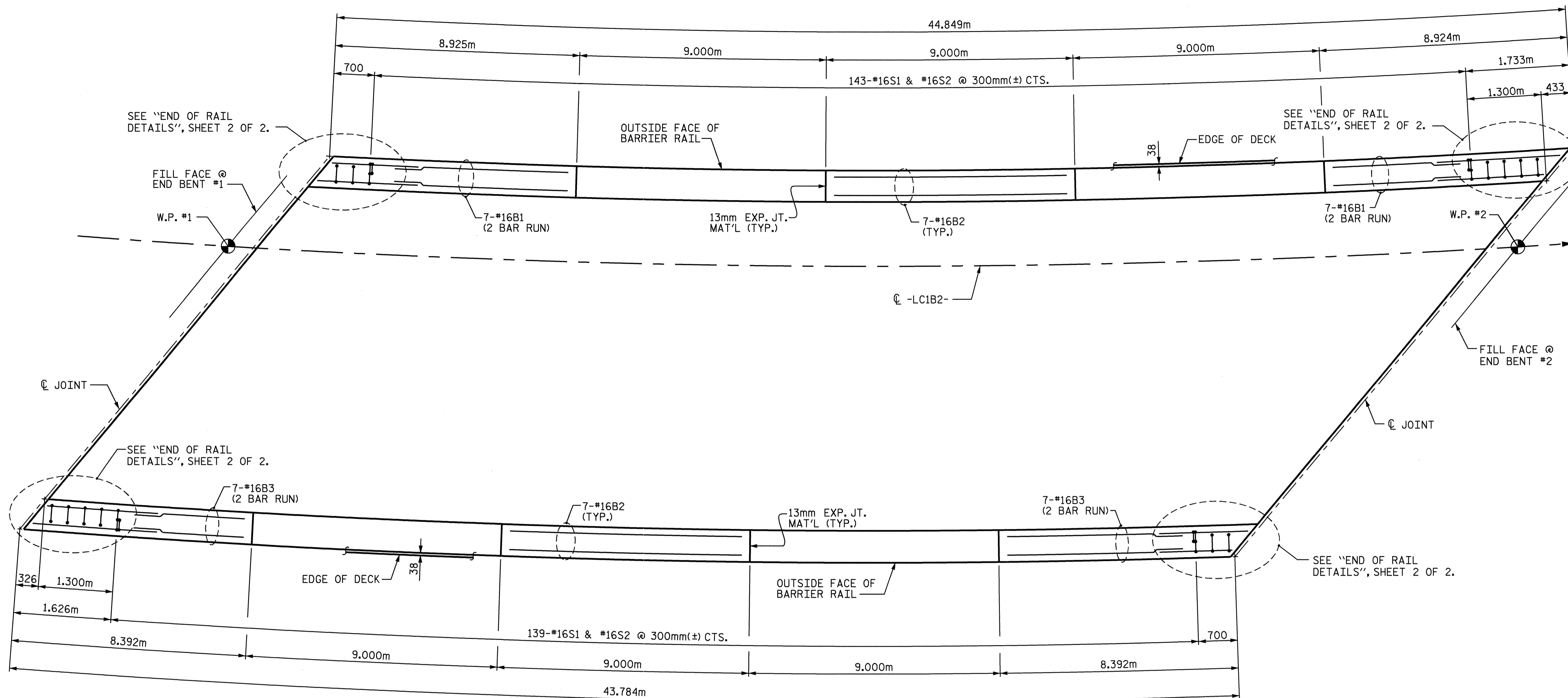
PLAN OF SPAN A DIMENSIONS ARE ARC LENGTHS ALONG OUTSIDE FACE OF BARRIER RAIL
