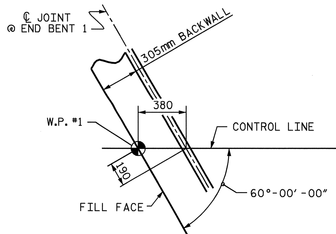
DETAIL A
