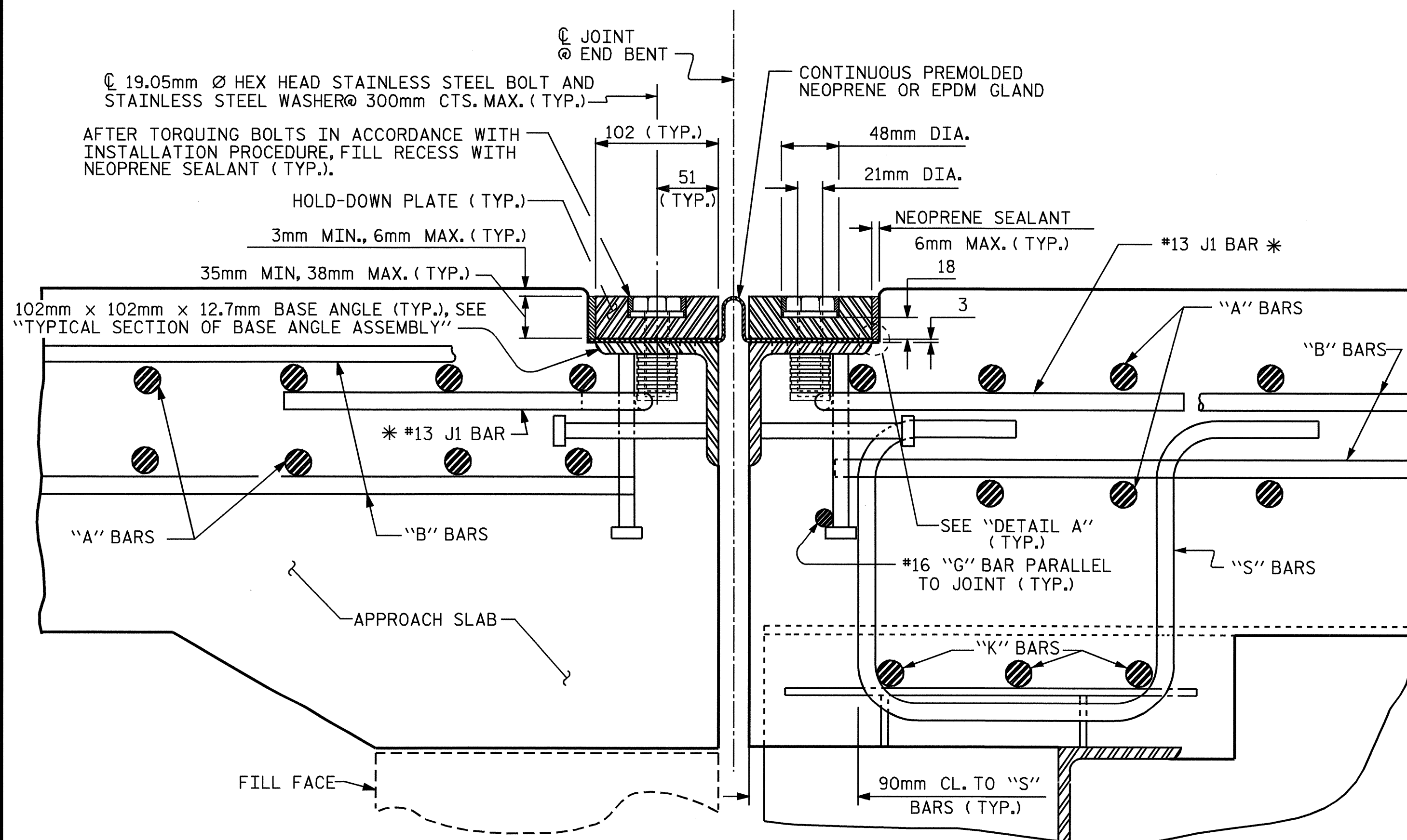
EXPANSION JOINT DETAILS (END BENT 1 SHOWN END BENT 2 SIMILAR)
