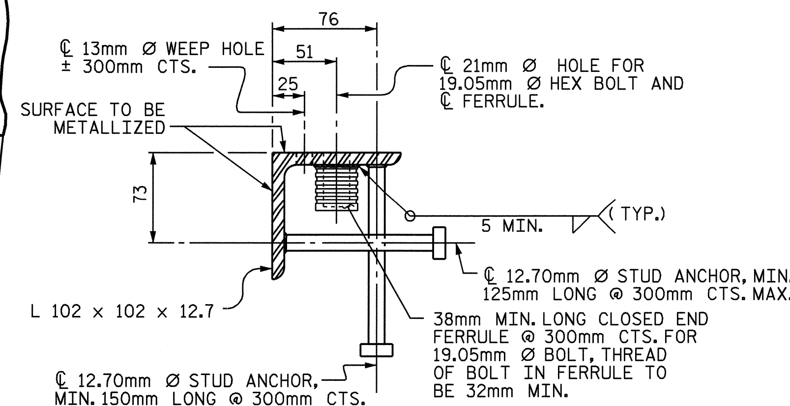
TYPICAL SECTION OF BASE ANGLE ASSEMBLY
