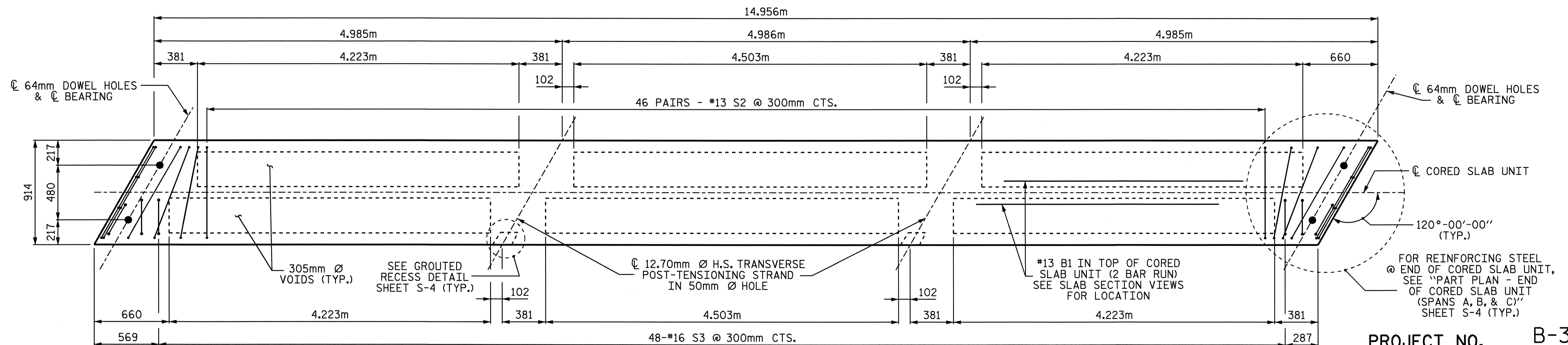
PLAN OF EXTERIOR CORED SLAB UNITS (TYP. SPANS A, B, & C)
