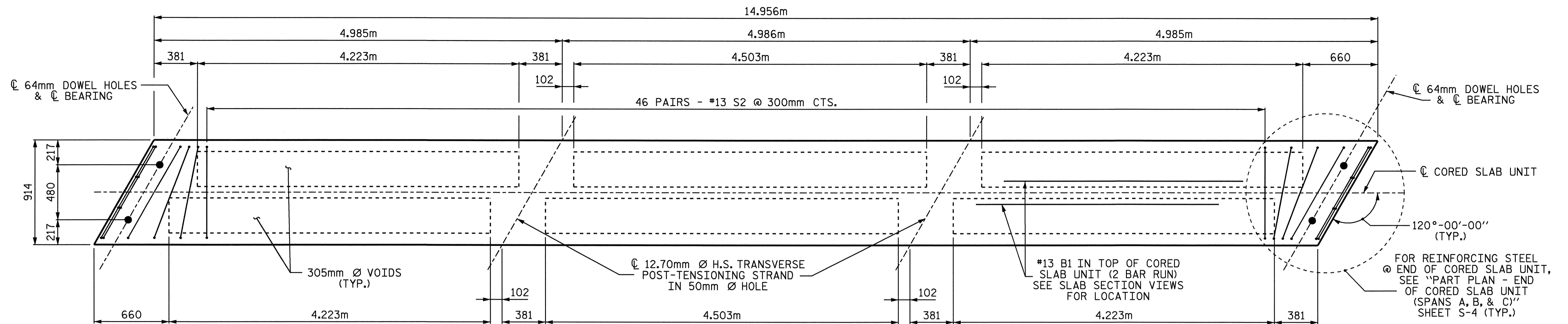
PLAN OF INTERIOR CORED SLAB UNITS (TYP. SPANS A, B, & C)
