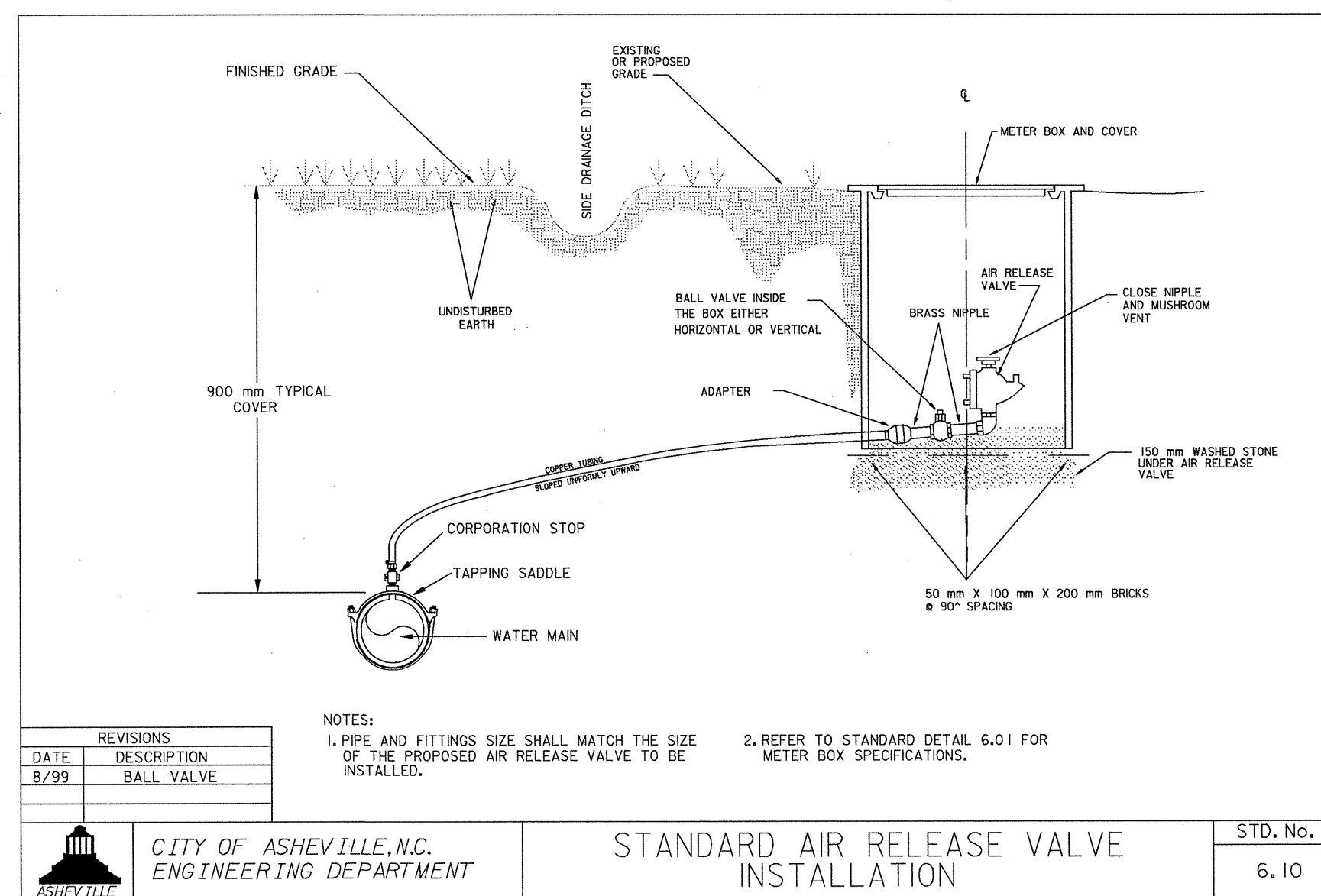
PRESSURE AIR RELEASE VALVE ASSEMBLY (ARV) 205
