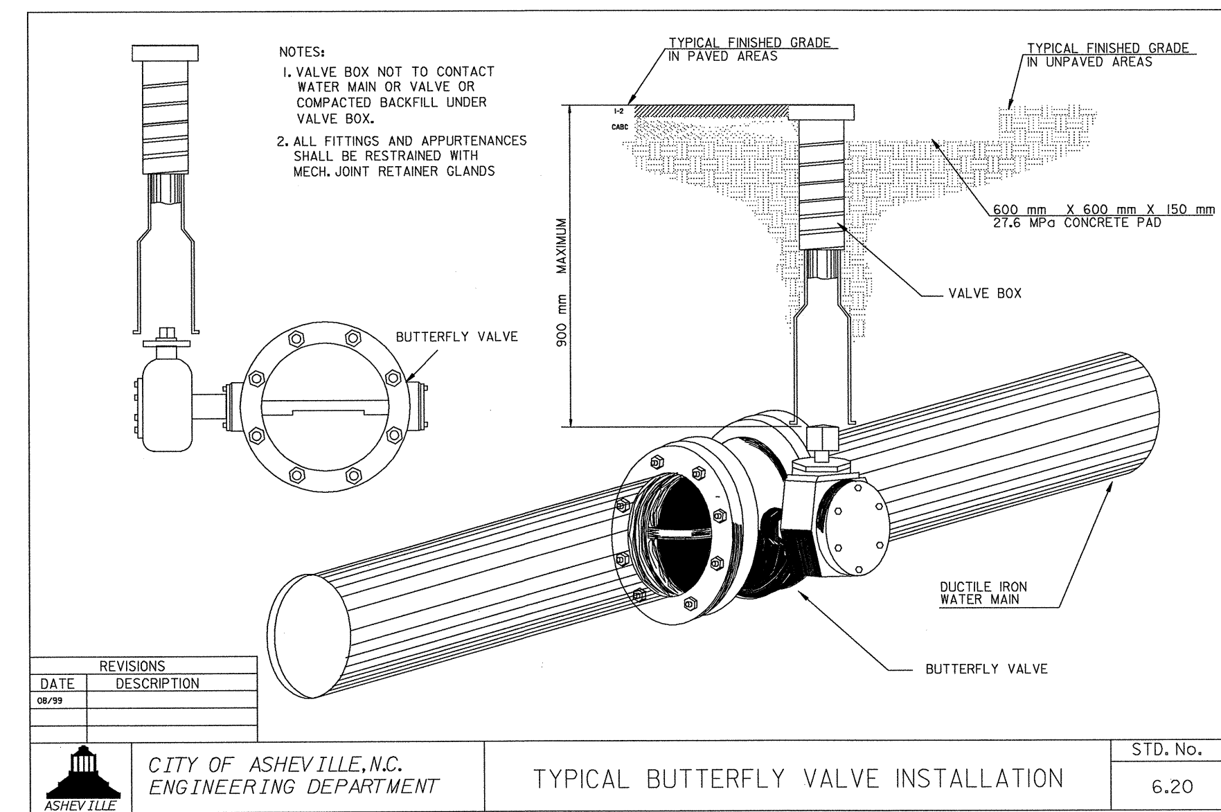
TYPICAL BUTTERFLY VALVE ASSEMBLY 208
