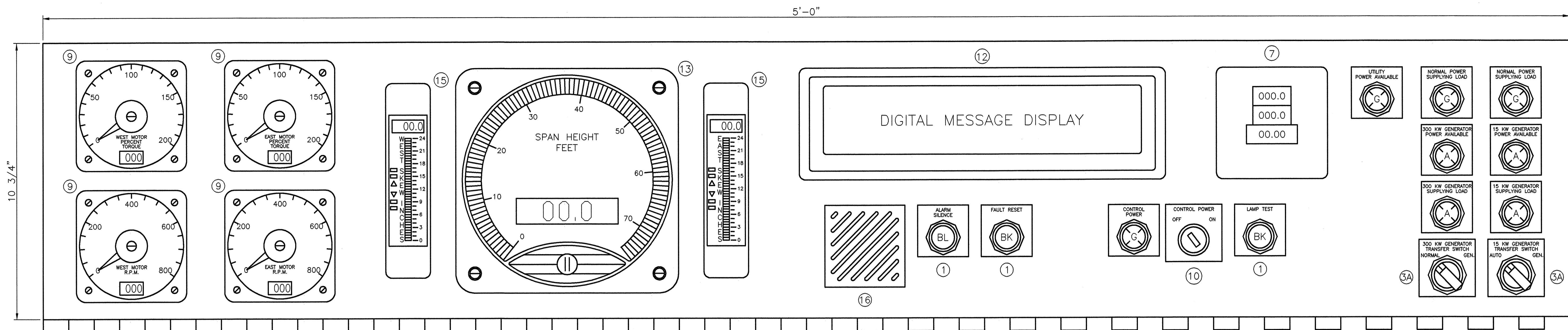
BRIDGE INDICATOR PANEL
