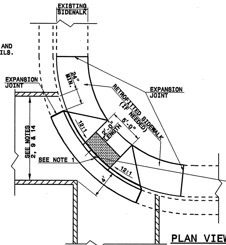
DETECTABLE WARNING DOMES
