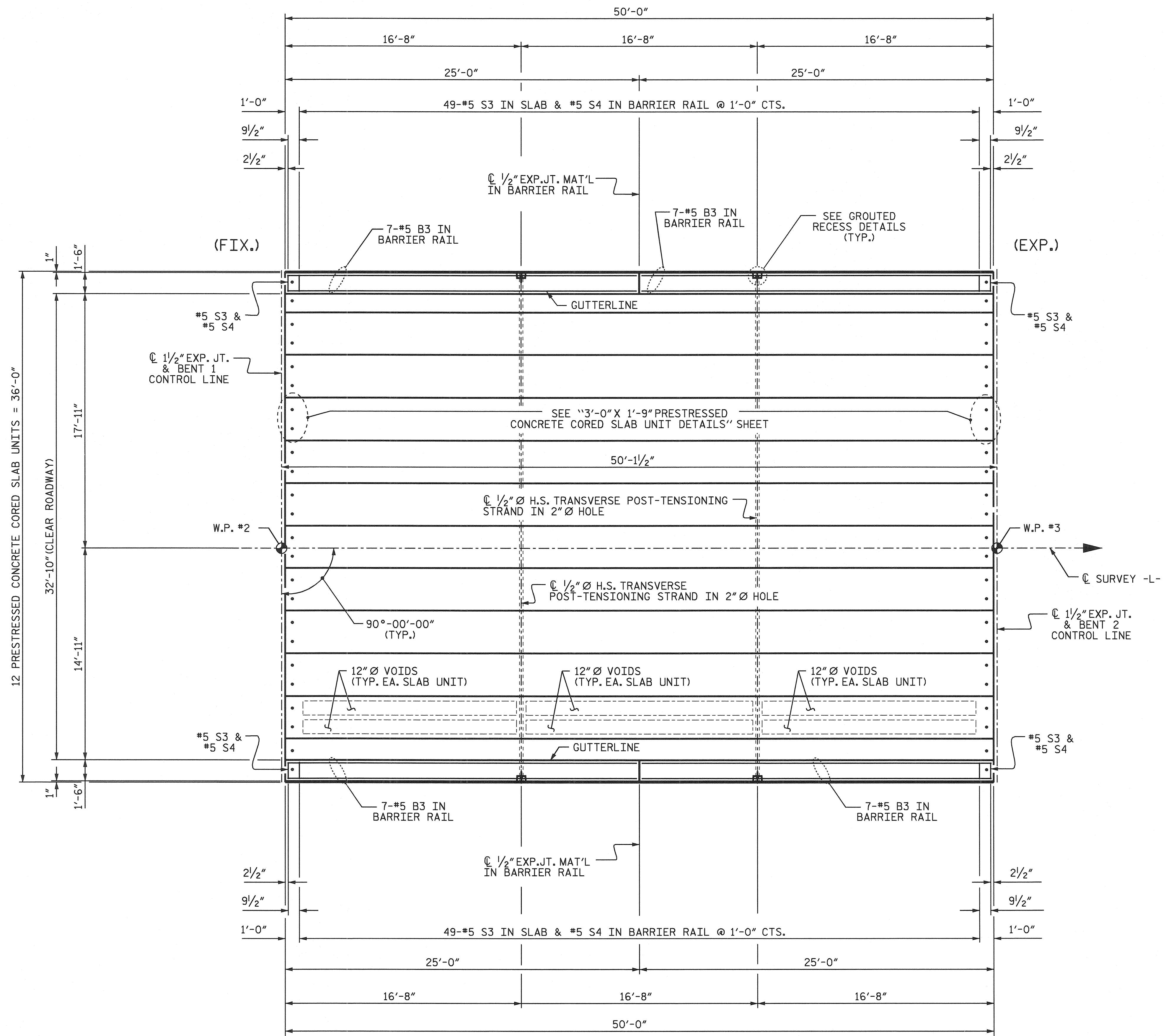
PLAN OF SPAN B
