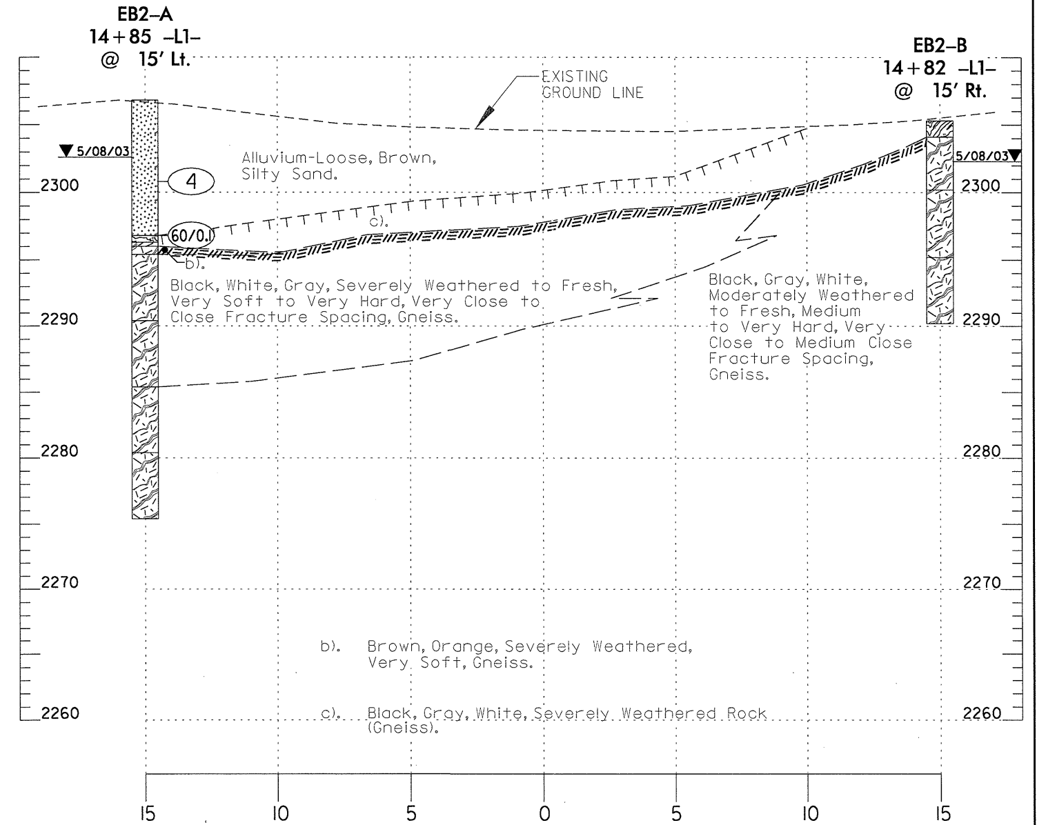
CROSS SECTION @ END BENT 2
