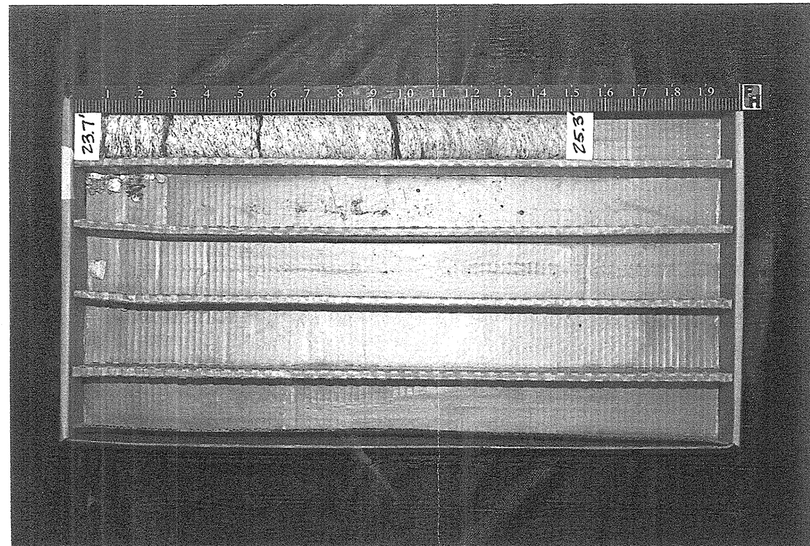
BORING EB1-B STA. 14+30 -L- @ 15.0 RIGHT BOX 2 of 2
