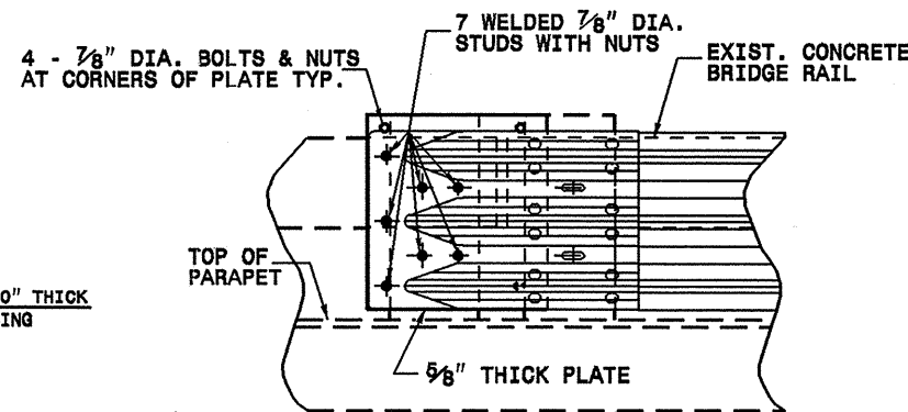
ELEVATION VIEW
