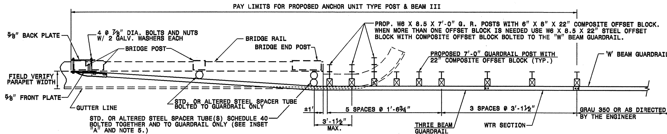
PLAN VIEW
