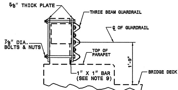
SECTION VIEW
