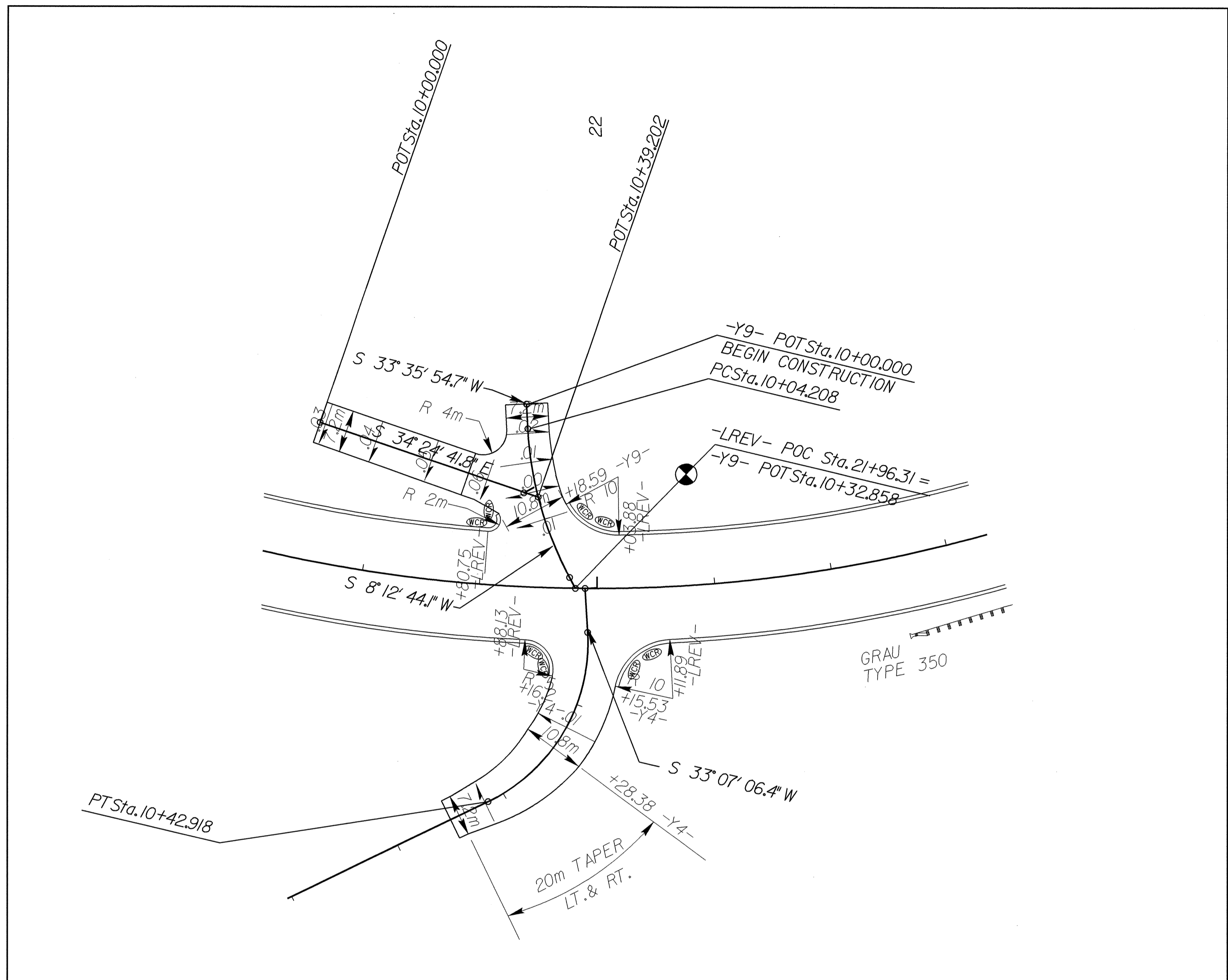
DETAIL OF INTERSECTION OF -LREV- & -Y4- & -Y9-
