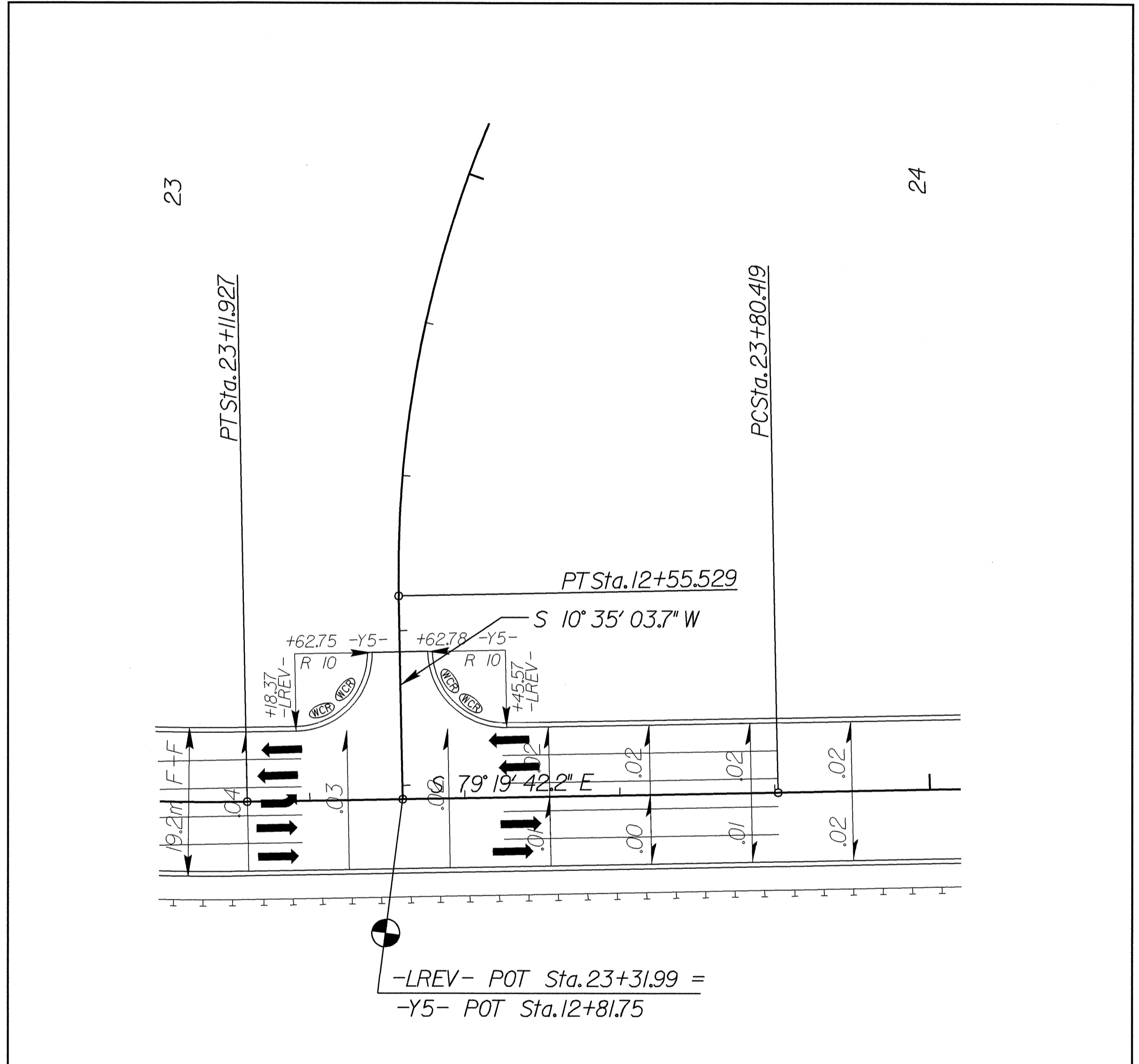
DETAIL OF INTERSECTION OF -LREV- & -Y5-
