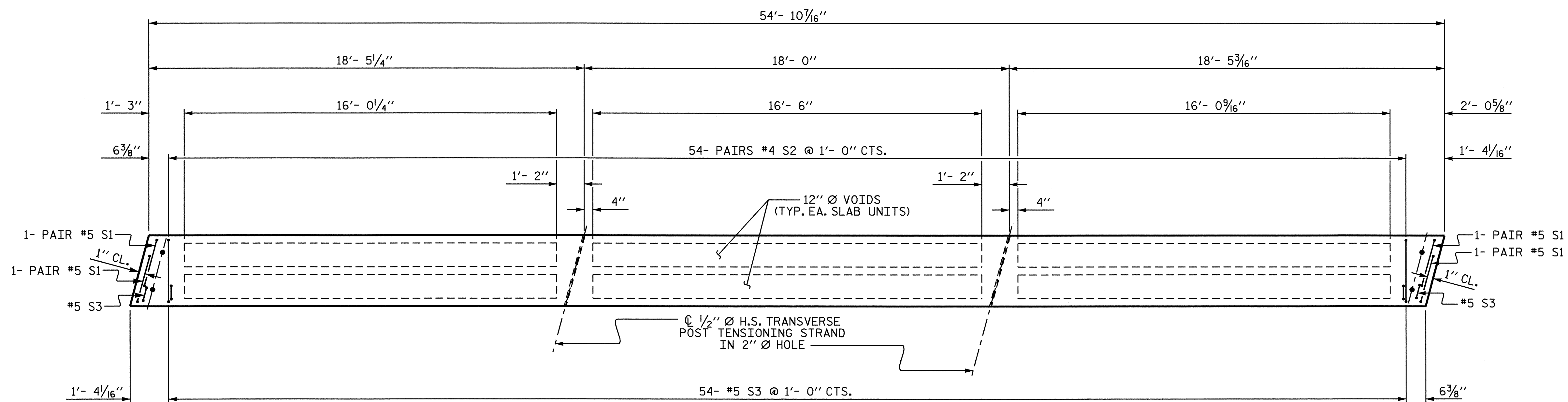
PLAN OF EXTERIOR CORED SLAB UNIT (SPAN "B")
