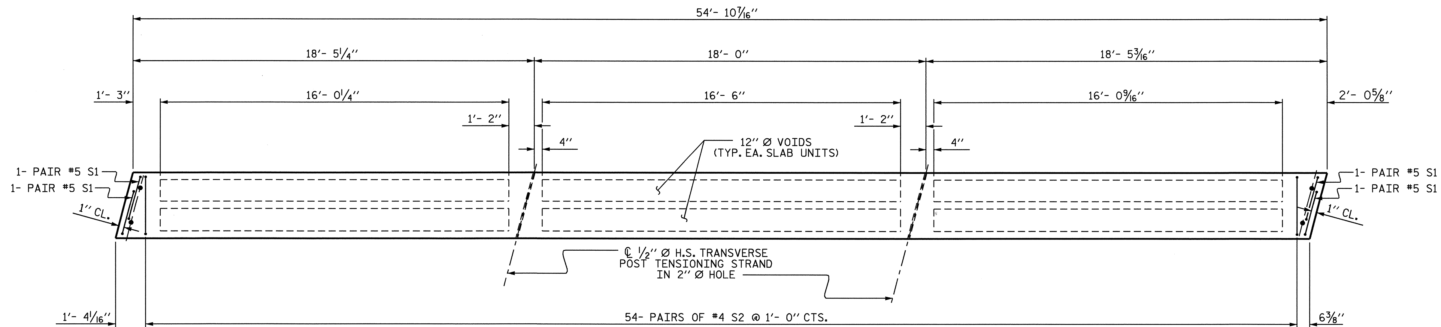
PLAN OF INTERIOR CORED SLAB UNIT (SPAN "B")
