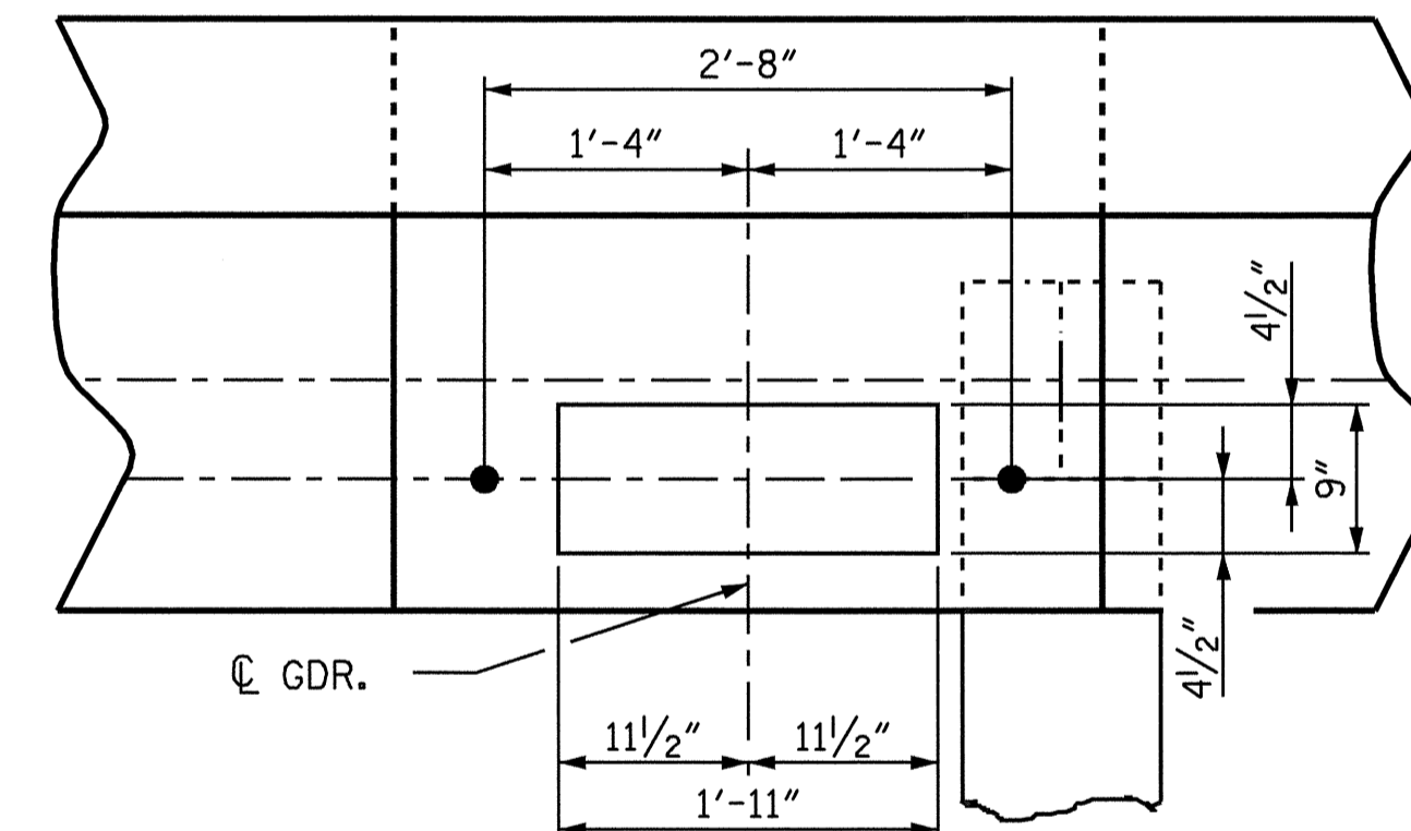
DETAIL A
