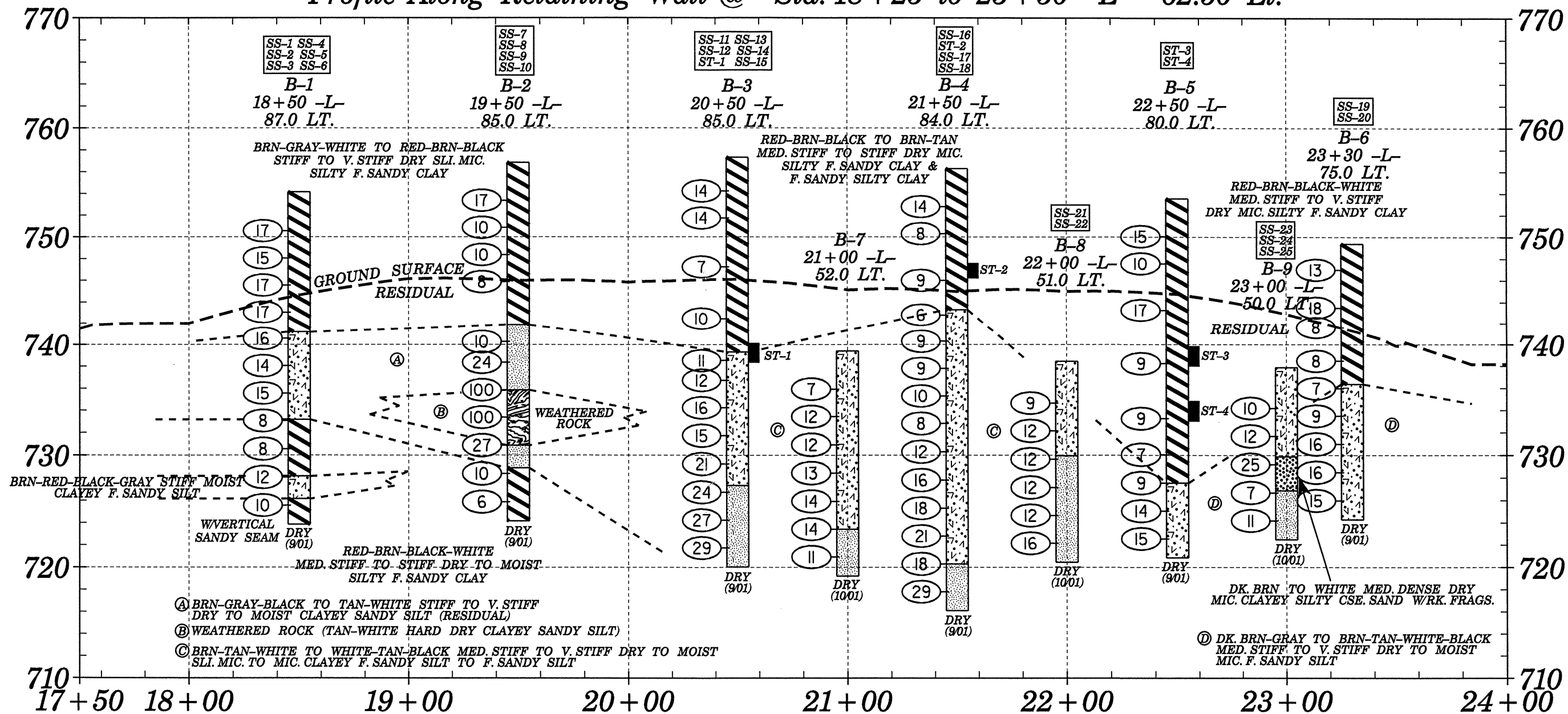
Profile Along Retaining Wall @ Sta. 18+25 to 23+50 -L- 62.50 Lt.
