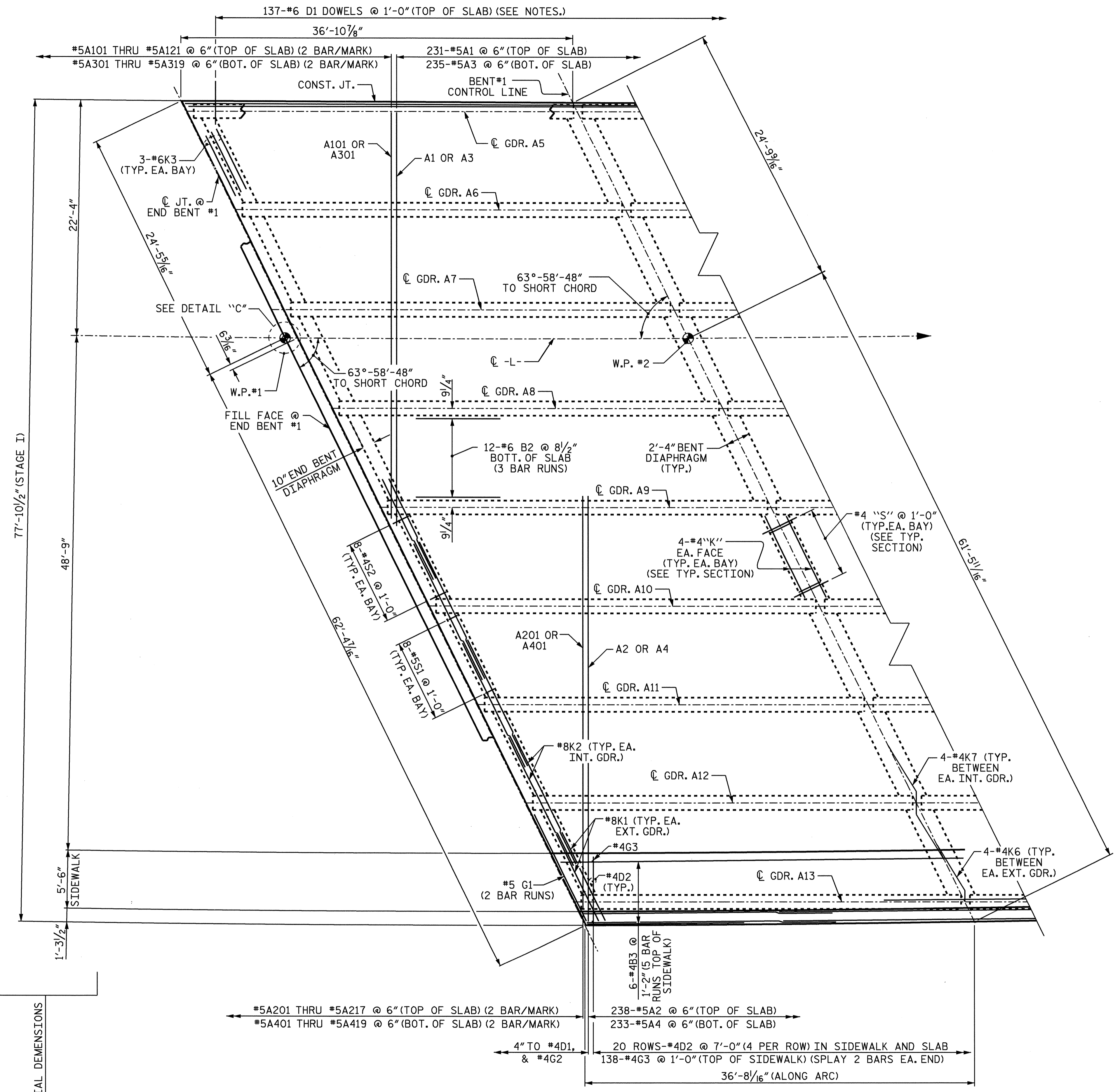
PLAN OF SPAN "A"
