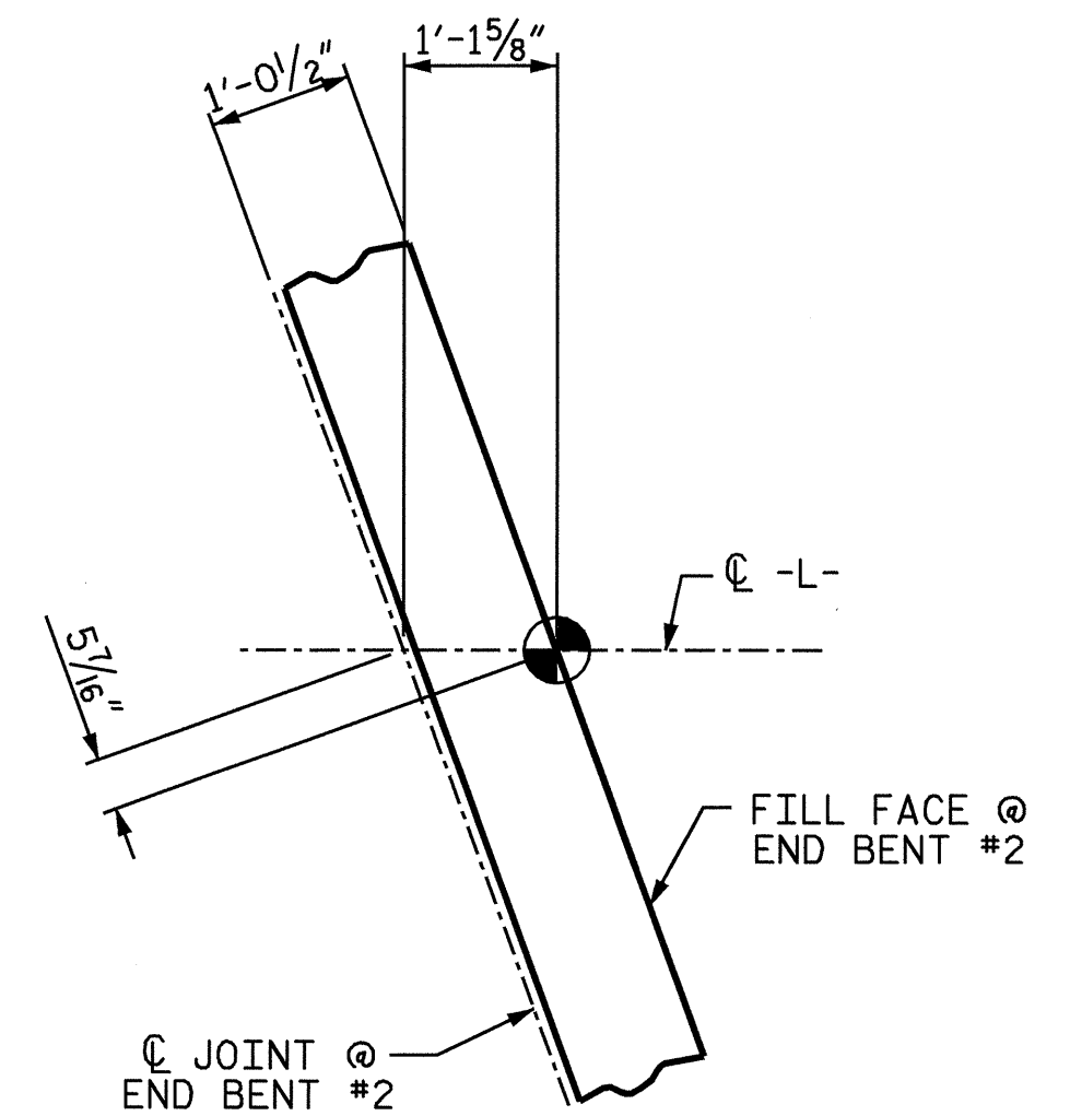
DETAIL "D"
